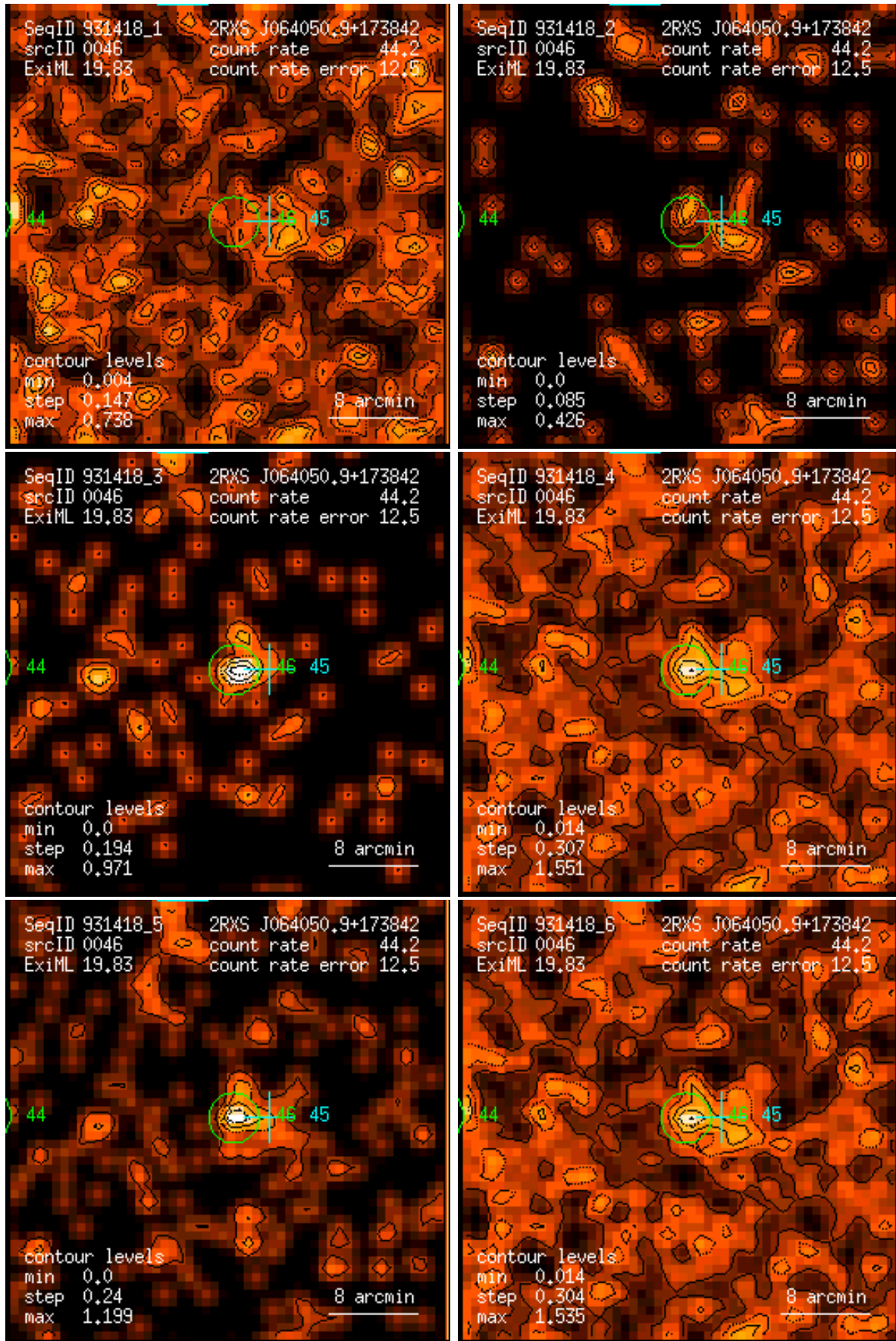
Figure 46: RASS 931418: detection 0046: band rate images, Gaussian filter: (1) PSPC channels 11 – 41, (2) 52 – 90, (3) 91 – 201, (4) 11 – 235, (5) 52 – 201, (6) 11 – 201. Broad band rates in counts/ks. Band rate contour levels in counts/ks/arcmin 2 .
