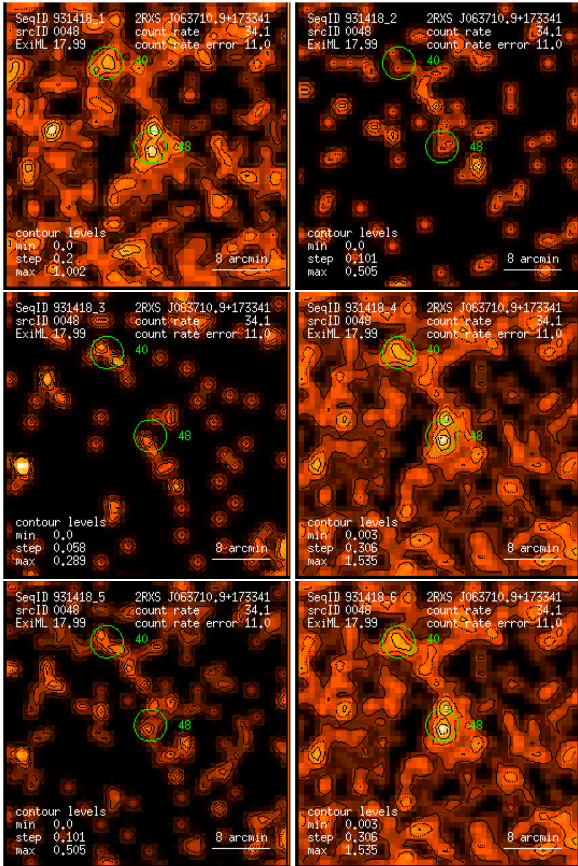
Figure 48: RASS 931418: detection 0048: band rate images, Gaussian filter: (1) PSPC channels 11 – 41, (2) 52 – 90, (3) 91 – 201, (4) 11 – 235, (5) 52 – 201, (6) 11 – 201. Broad band rates in counts/ks. Band rate contour levels in counts/ks/arcmin 2 .
