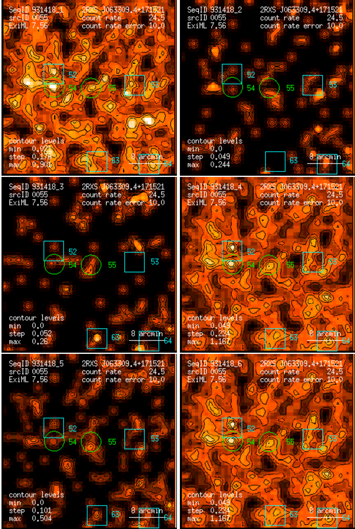
Figure 55: RASS 931418: detection 0055: band rate images, Gaussian filter: (1) PSPC channels 11 – 41, (2) 52 – 90, (3) 91 – 201, (4) 11 – 235, (5) 52 – 201, (6) 11 – 201. Broad band rates in counts/ks. Band rate contour levels in counts/ks/arcmin 2 .
