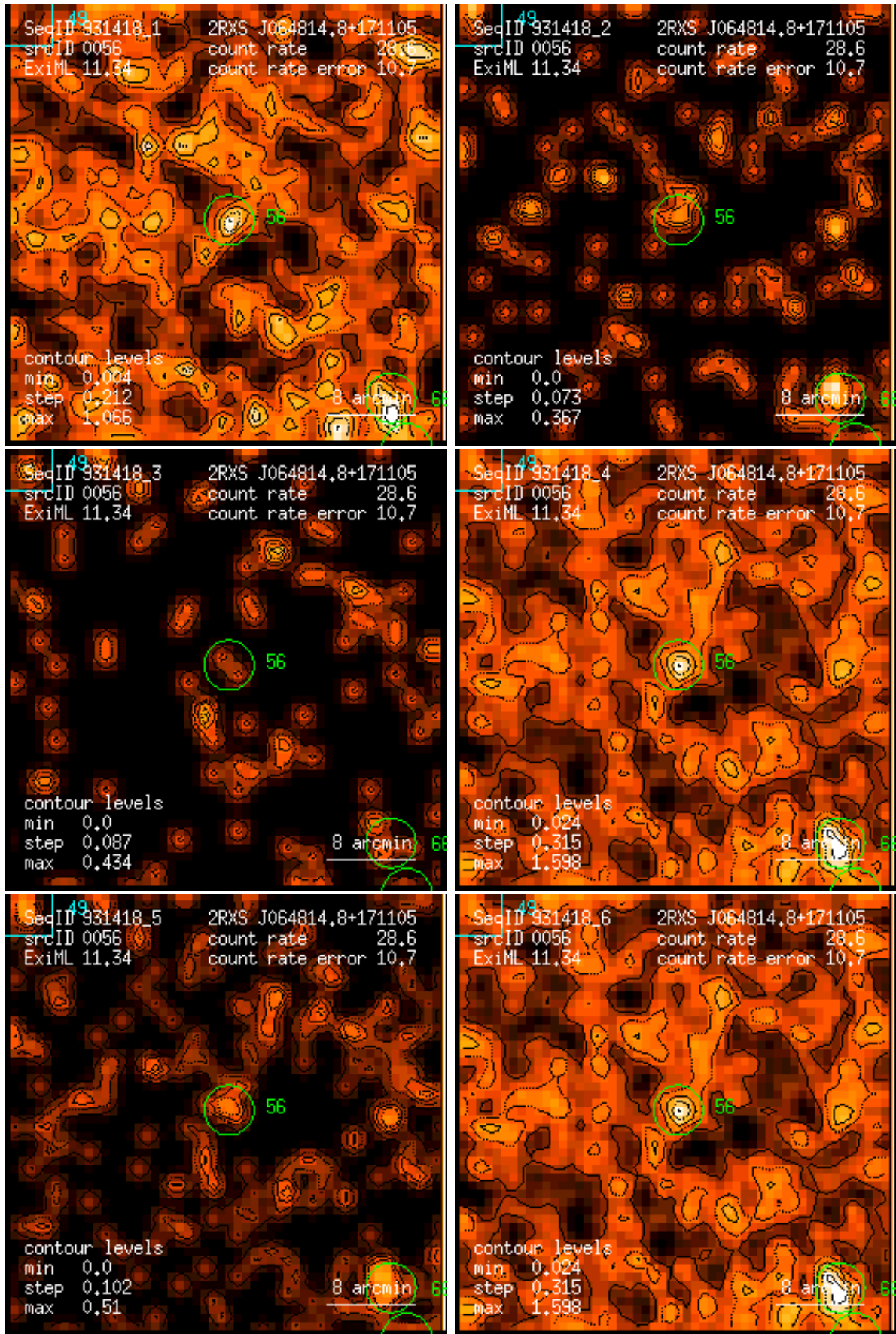
Figure 56: RASS 931418: detection 0056: band rate images, Gaussian filter: (1) PSPC channels 11 – 41, (2) 52 – 90, (3) 91 – 201, (4) 11 – 235, (5) 52 – 201, (6) 11 – 201. Broad band rates in counts/ks. Band rate contour levels in counts/ks/arcmin 2 .
