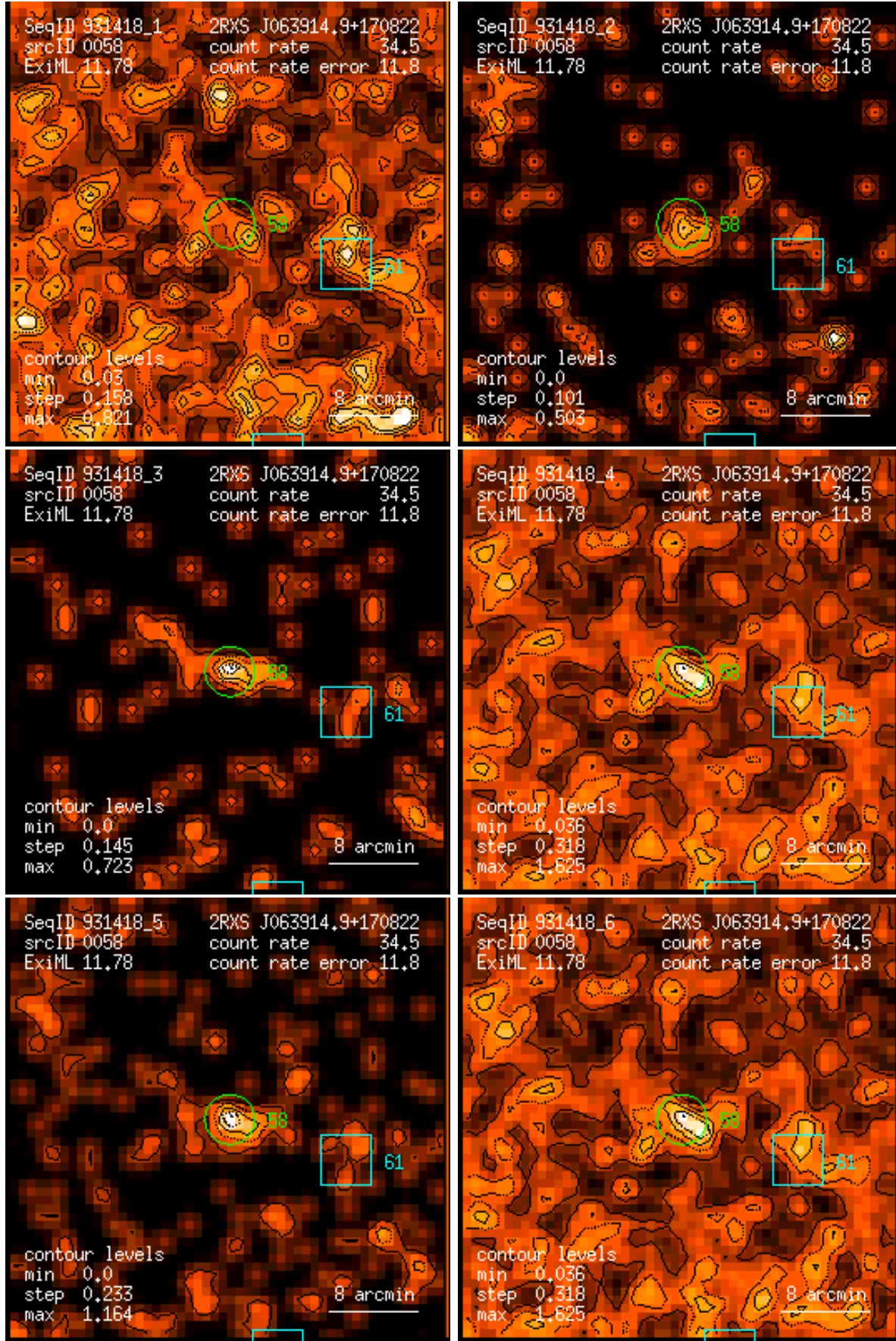
Figure 58: RASS 931418: detection 0058: band rate images, Gaussian filter: (1) PSPC channels 11 – 41, (2) 52 – 90, (3) 91 – 201, (4) 11 – 235, (5) 52 – 201, (6) 11 – 201. Broad band rates in counts/ks. Band rate contour levels in counts/ks/arcmin 2 .
