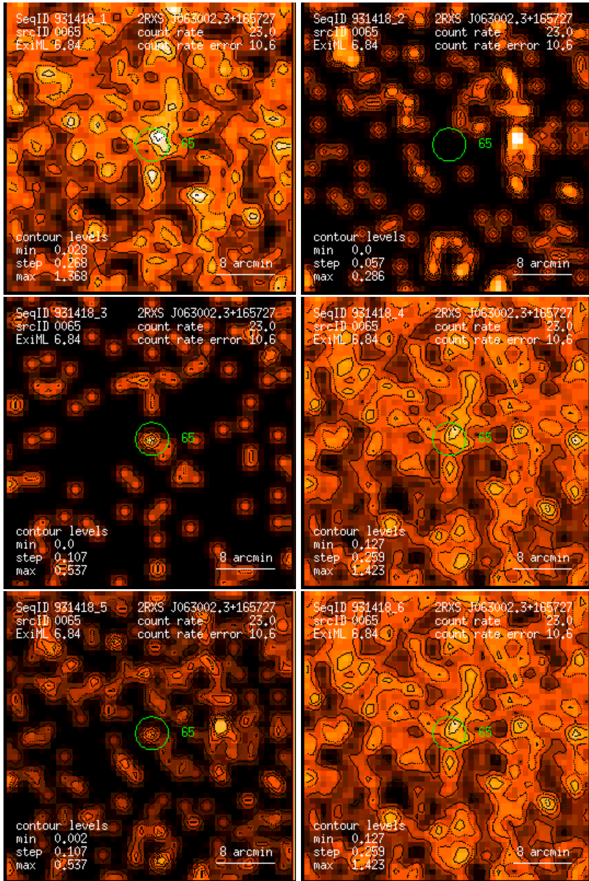
Figure 65: RASS 931418: detection 0065: band rate images, Gaussian filter: (1) PSPC channels 11 – 41, (2) 52 – 90, (3) 91 – 201, (4) 11 – 235, (5) 52 – 201, (6) 11 – 201. Broad band rates in counts/ks. Band rate contour levels in counts/ks/arcmin 2 .
