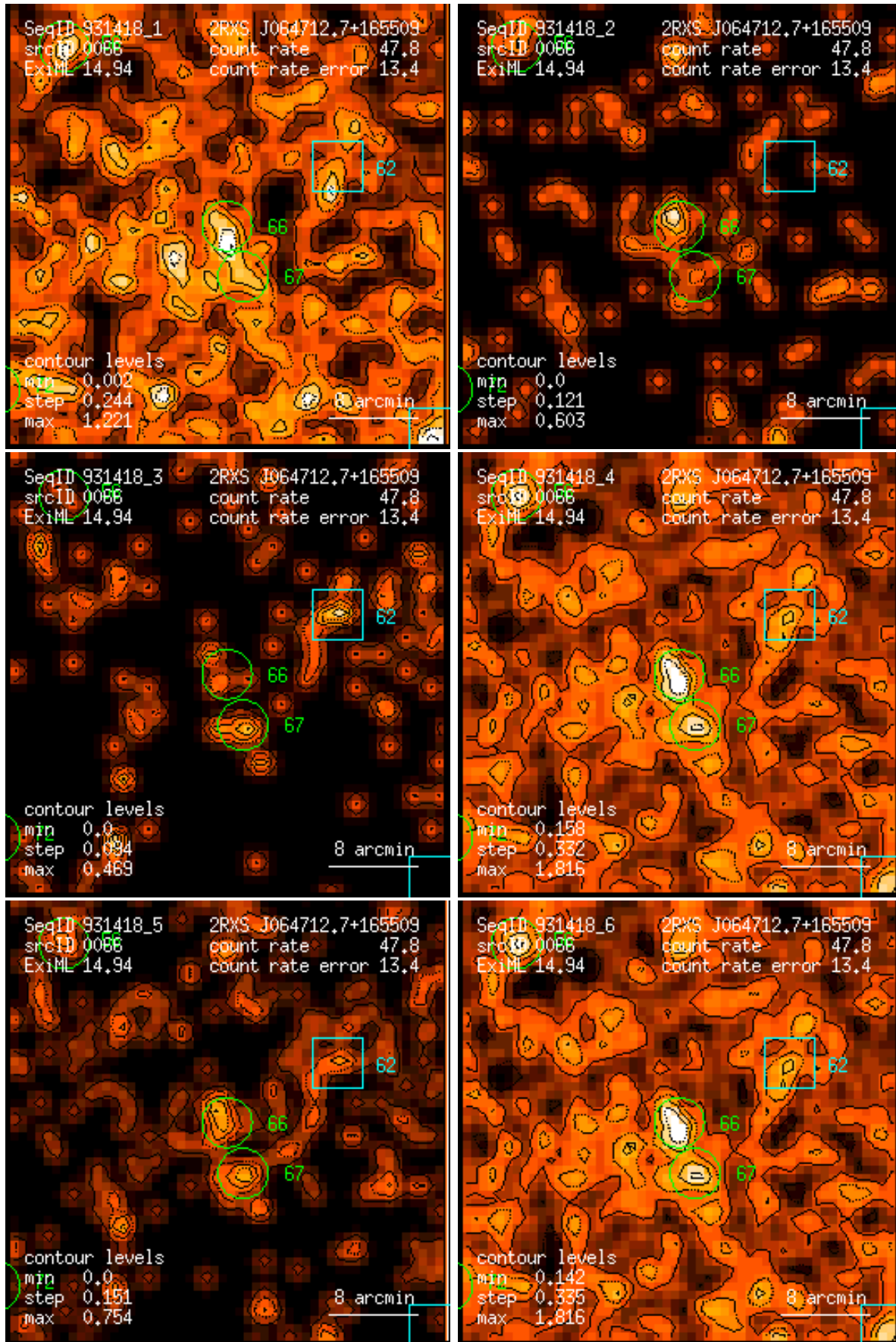
Figure 66: RASS 931418: detection 0066: band rate images, Gaussian filter: (1) PSPC channels 11 – 41, (2) 52 – 90, (3) 91 – 201, (4) 11 – 235, (5) 52 – 201, (6) 11 – 201. Broad band rates in counts/ks. Band rate contour levels in counts/ks/arcmin 2 .
