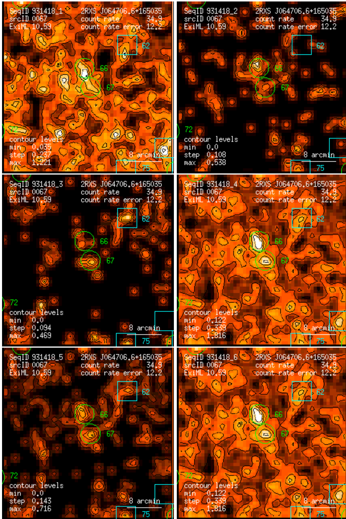
Figure 67: RASS 931418: detection 0067: band rate images, Gaussian filter: (1) PSPC channels 11 – 41, (2) 52 – 90, (3) 91 – 201, (4) 11 – 235, (5) 52 – 201, (6) 11 – 201. Broad band rates in counts/ks. Band rate contour levels in counts/ks/arcmin 2 .
