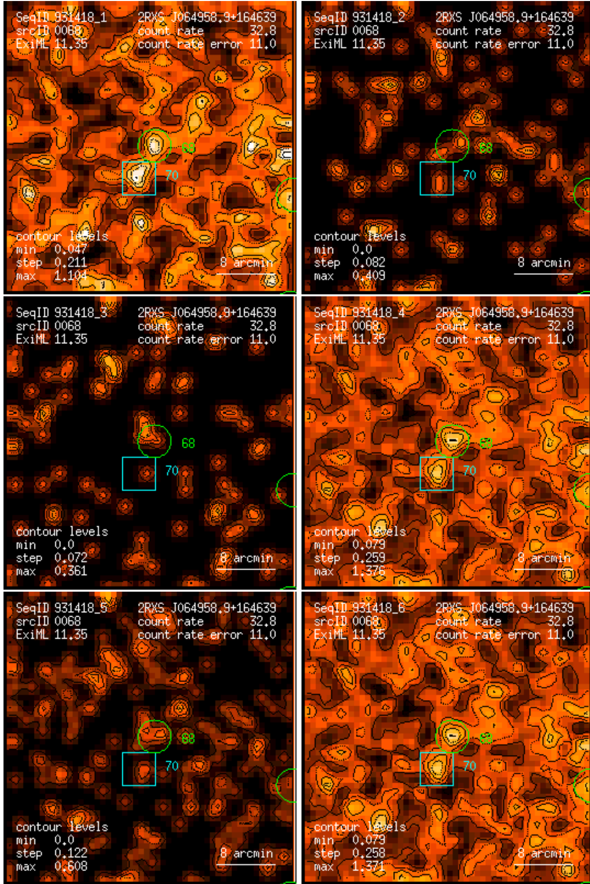
Figure 68: RASS 931418: detection 0068: band rate images, Gaussian filter: (1) PSPC channels 11 – 41, (2) 52 – 90, (3) 91 – 201, (4) 11 – 235, (5) 52 – 201, (6) 11 – 201. Broad band rates in counts/ks. Band rate contour levels in counts/ks/arcmin 2 .
