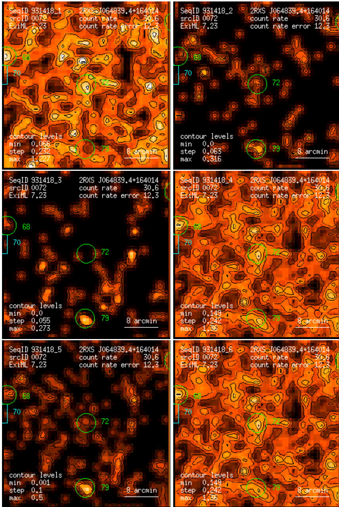
Figure 72: RASS 931418: detection 0072: band rate images, Gaussian filter: (1) PSPC channels 11 – 41, (2) 52 – 90, (3) 91 – 201, (4) 11 – 235, (5) 52 – 201, (6) 11 – 201. Broad band rates in counts/ks. Band rate contour levels in counts/ks/arcmin 2 .
