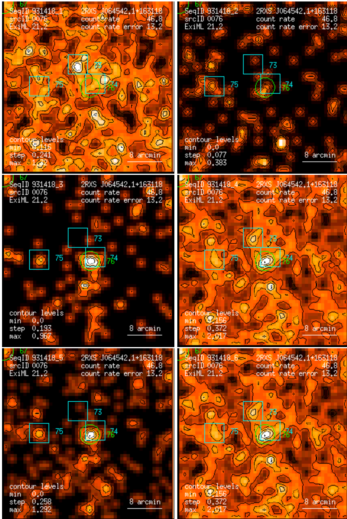
Figure 76: RASS 931418: detection 0076: band rate images, Gaussian filter: (1) PSPC channels 11 – 41, (2) 52 – 90, (3) 91 – 201, (4) 11 – 235, (5) 52 – 201, (6) 11 – 201. Broad band rates in counts/ks. Band rate contour levels in counts/ks/arcmin 2 .
