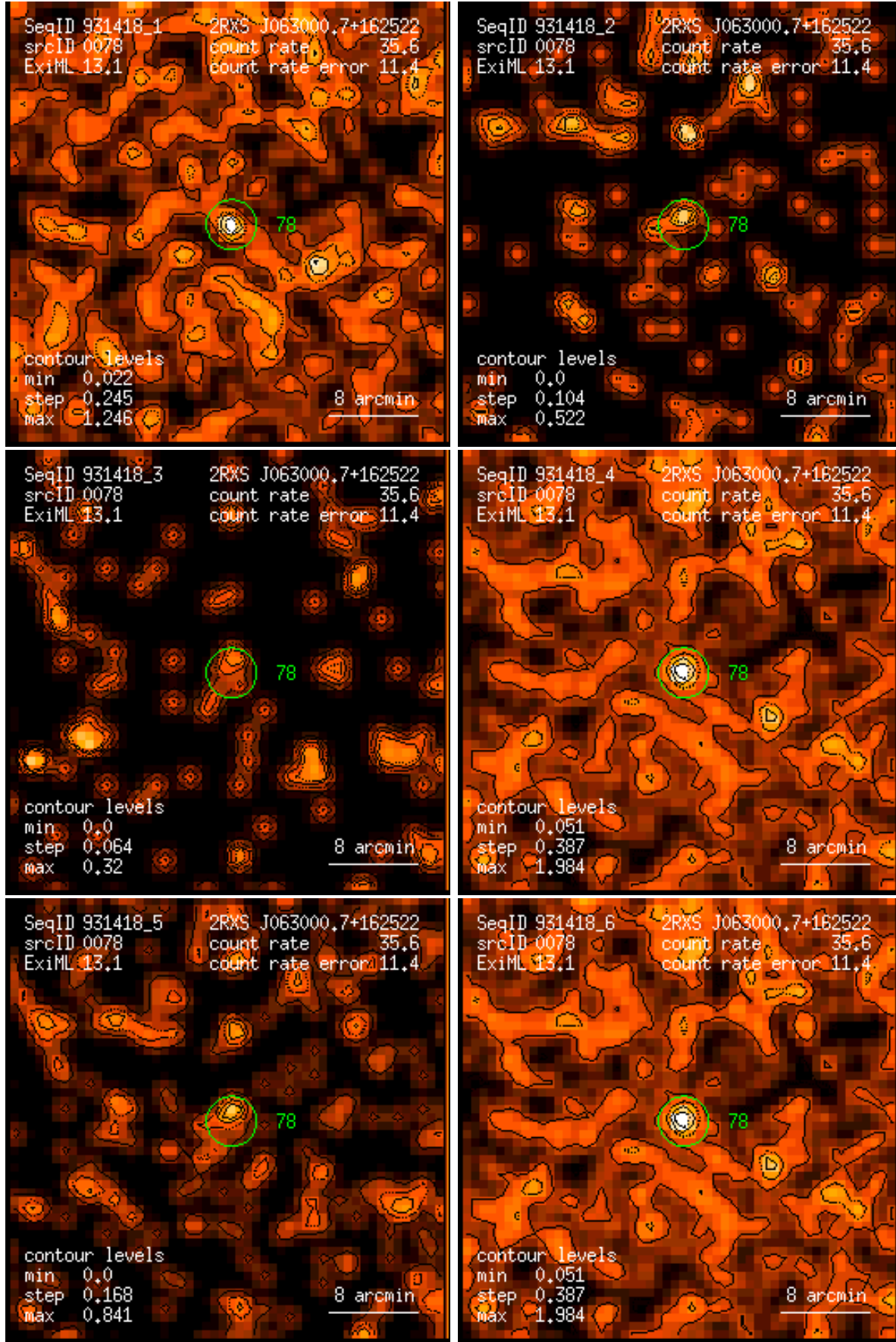
Figure 78: RASS 931418: detection 0078: band rate images, Gaussian filter: (1) PSPC channels 11 – 41, (2) 52 – 90, (3) 91 – 201, (4) 11 – 235, (5) 52 – 201, (6) 11 – 201. Broad band rates in counts/ks. Band rate contour levels in counts/ks/arcmin 2 .
