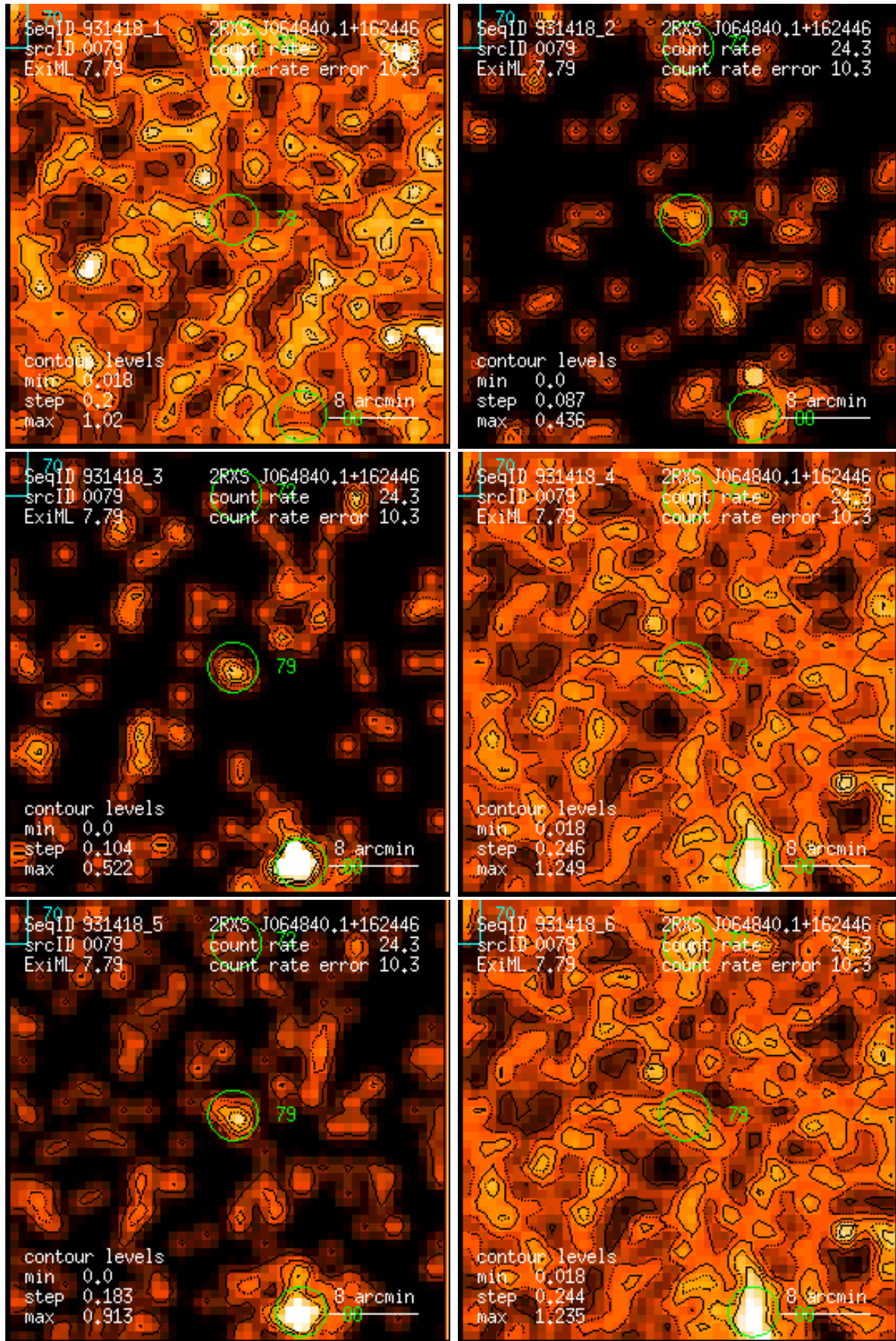
Figure 79: RASS 931418: detection 0079: band rate images, Gaussian filter: (1) PSPC channels 11 – 41, (2) 52 – 90, (3) 91 – 201, (4) 11 – 235, (5) 52 – 201, (6) 11 – 201. Broad band rates in counts/ks. Band rate contour levels in counts/ks/arcmin 2 .
