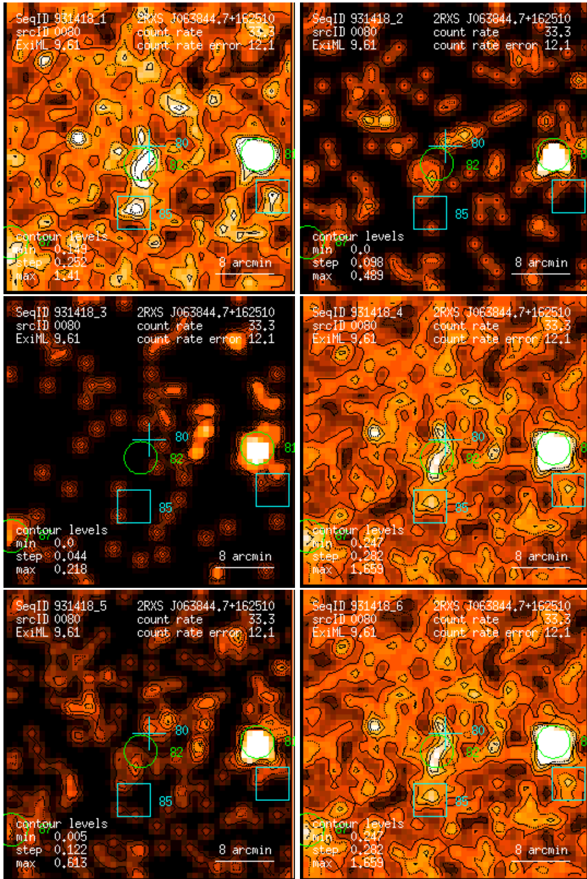
Figure 80: RASS 931418: detection 0080: band rate images, Gaussian filter: (1) PSPC channels 11 – 41, (2) 52 – 90, (3) 91 – 201, (4) 11 – 235, (5) 52 – 201, (6) 11 – 201. Broad band rates in counts/ks. Band rate contour levels in counts/ks/arcmin 2 .
