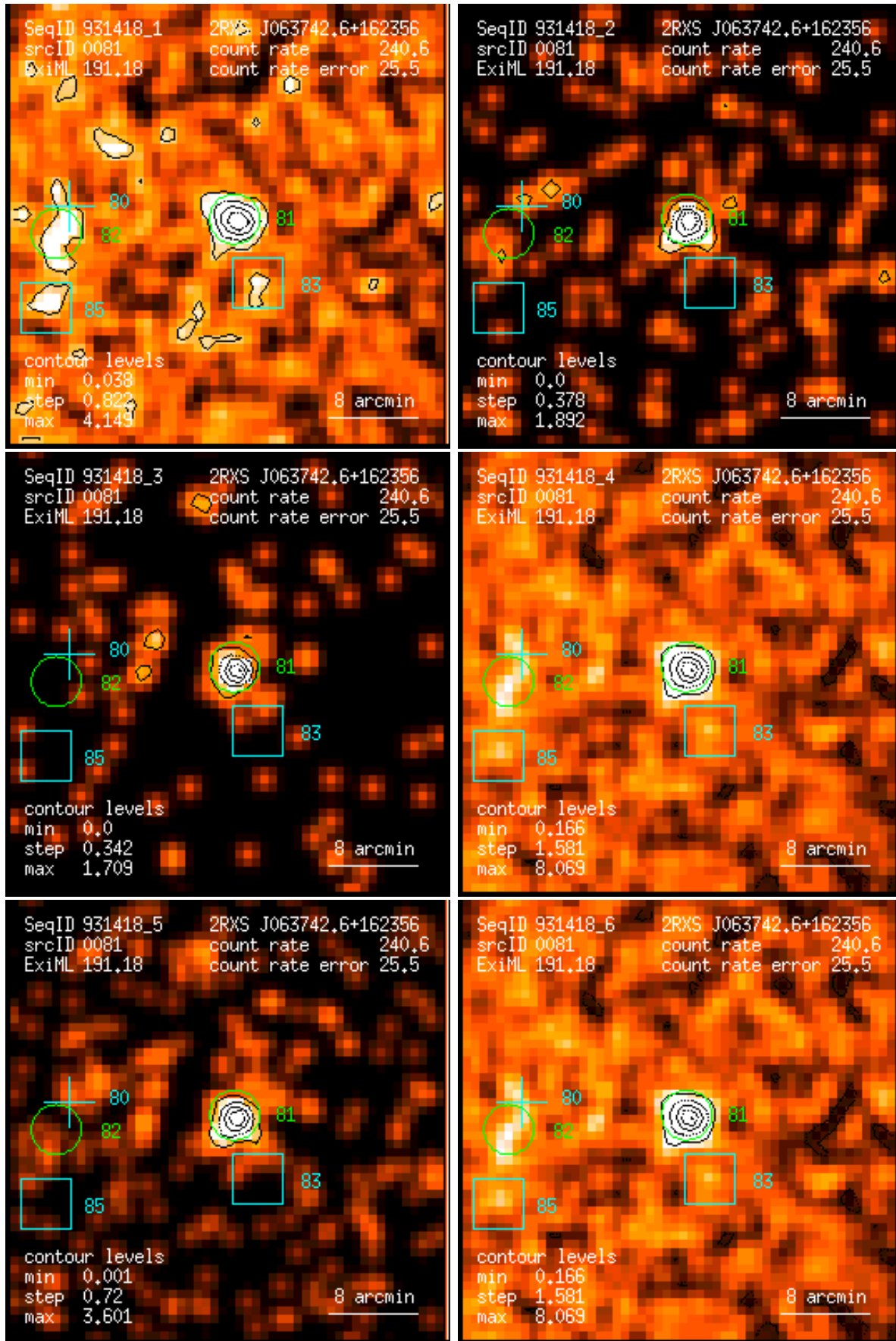
Figure 81: RASS 931418: detection 0081: band rate images, Gaussian filter: (1) PSPC channels 11 – 41, (2) 52 – 90, (3) 91 – 201, (4) 11 – 235, (5) 52 – 201, (6) 11 – 201. Broad band rates in counts/ks. Band rate contour levels in counts/ks/arcmin 2 .
