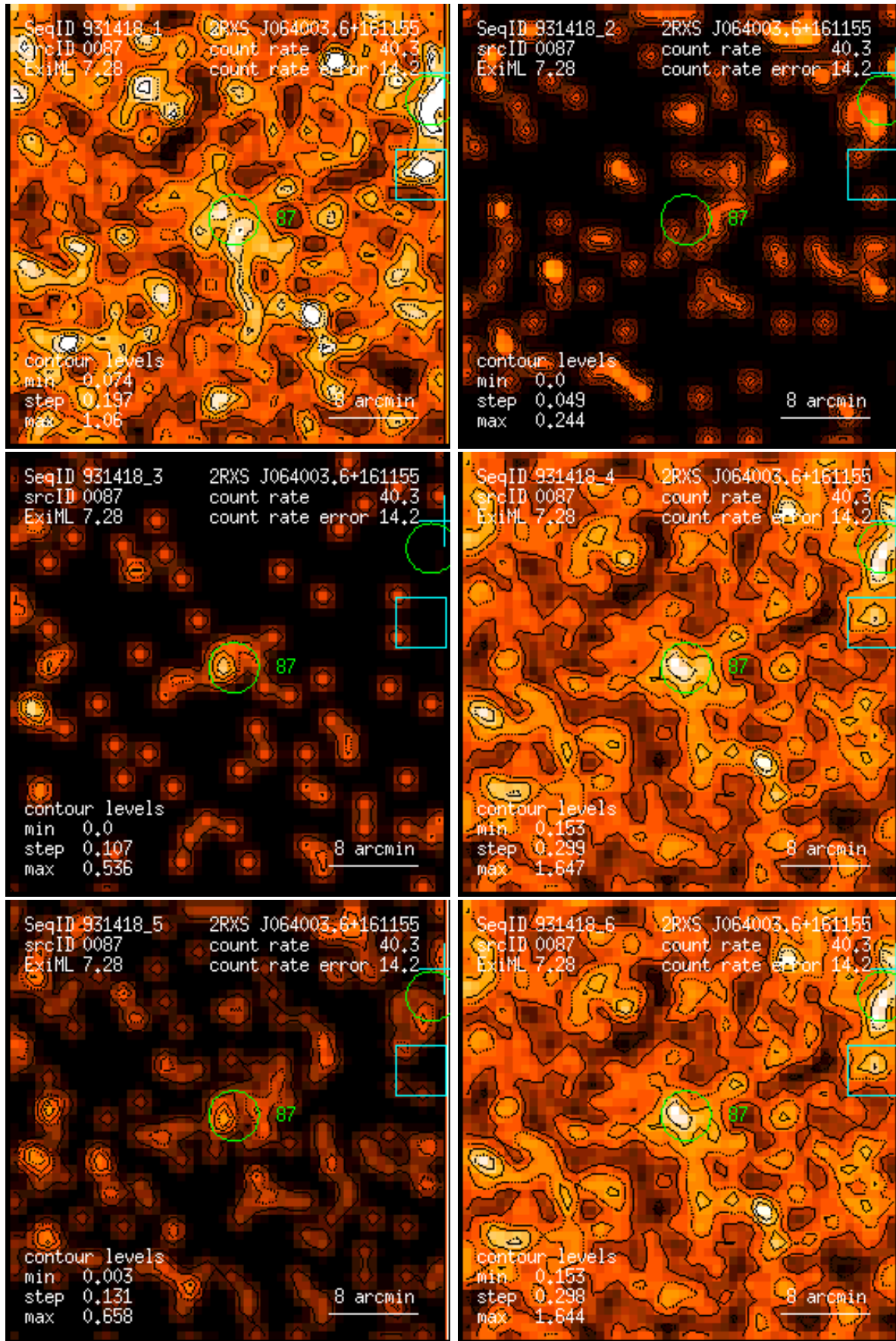
Figure 87: RASS 931418: detection 0087: band rate images, Gaussian filter: (1) PSPC channels 11 – 41, (2) 52 – 90, (3) 91 – 201, (4) 11 – 235, (5) 52 – 201, (6) 11 – 201. Broad band rates in counts/ks. Band rate contour levels in counts/ks/arcmin 2 .
