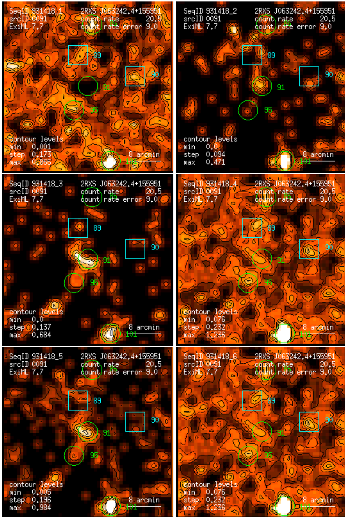
Figure 91: RASS 931418: detection 0091: band rate images, Gaussian filter: (1) PSPC channels 11 – 41, (2) 52 – 90, (3) 91 – 201, (4) 11 – 235, (5) 52 – 201, (6) 11 – 201. Broad band rates in counts/ks. Band rate contour levels in counts/ks/arcmin 2 .
