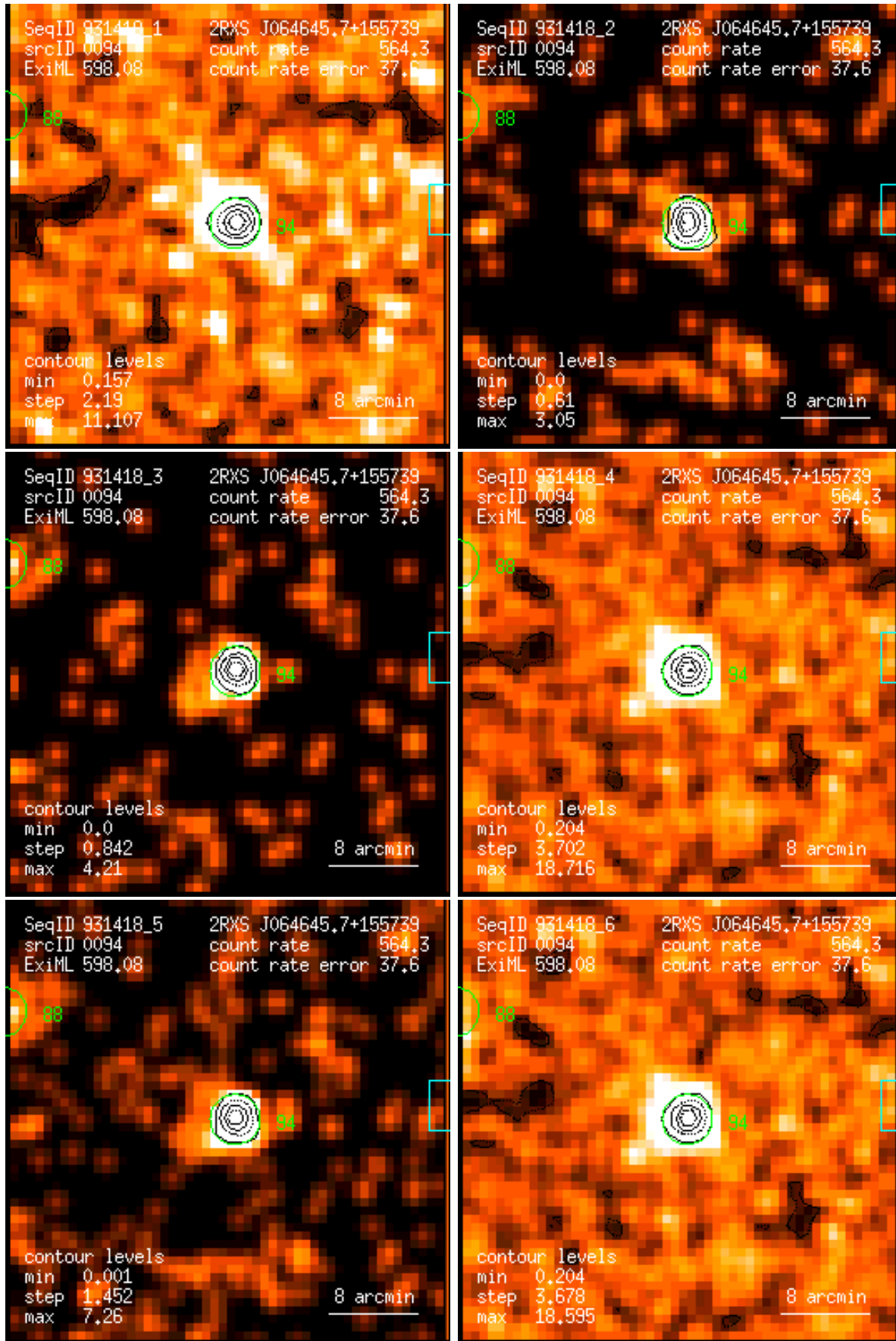
Figure 94: RASS 931418: detection 0094: band rate images, Gaussian filter: (1) PSPC channels 11 – 41, (2) 52 – 90, (3) 91 – 201, (4) 11 – 235, (5) 52 – 201, (6) 11 – 201. Broad band rates in counts/ks. Band rate contour levels in counts/ks/arcmin 2 .
