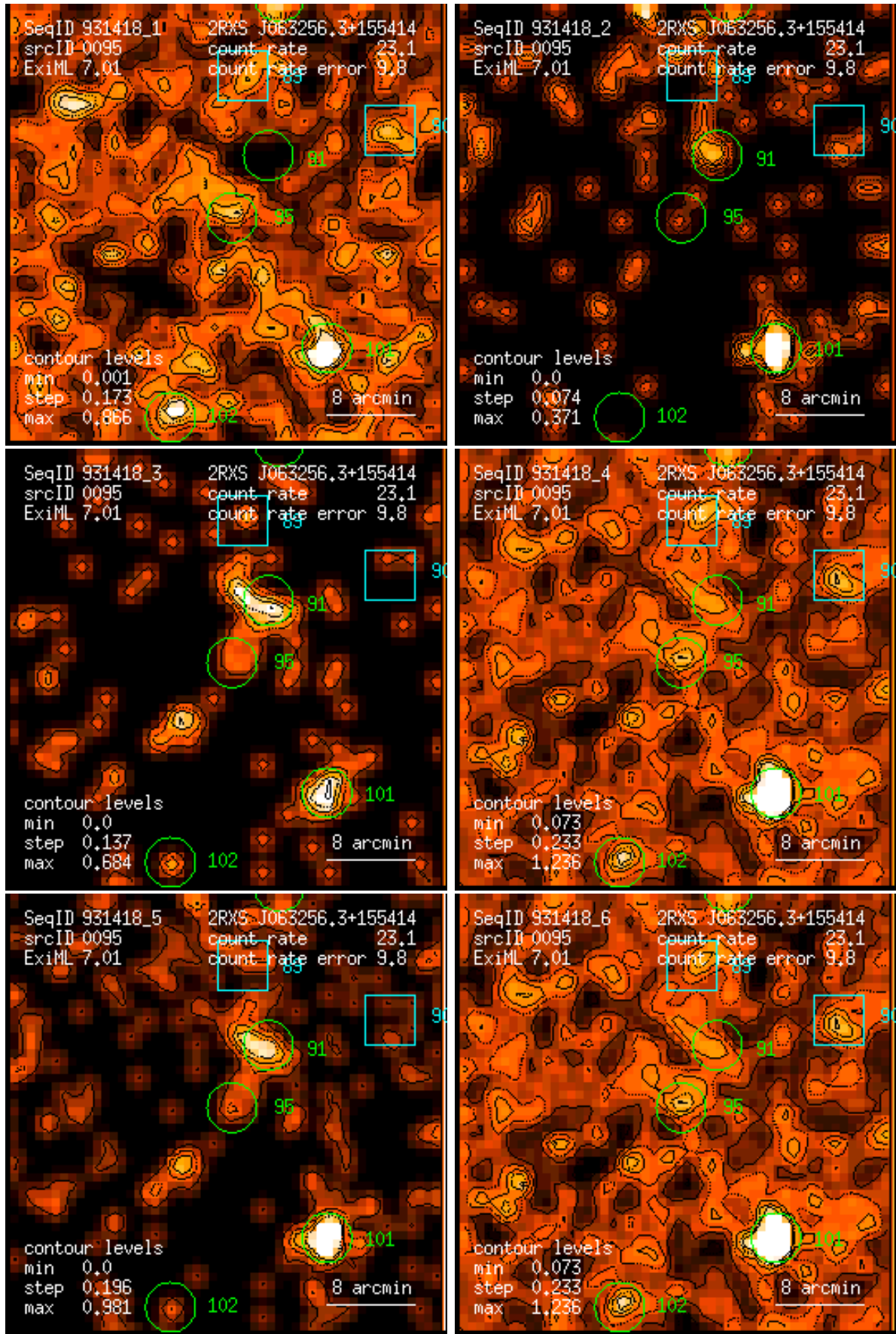
Figure 95: RASS 931418: detection 0095: band rate images, Gaussian filter: (1) PSPC channels 11 – 41, (2) 52 – 90, (3) 91 – 201, (4) 11 – 235, (5) 52 – 201, (6) 11 – 201. Broad band rates in counts/ks. Band rate contour levels in counts/ks/arcmin 2 .
