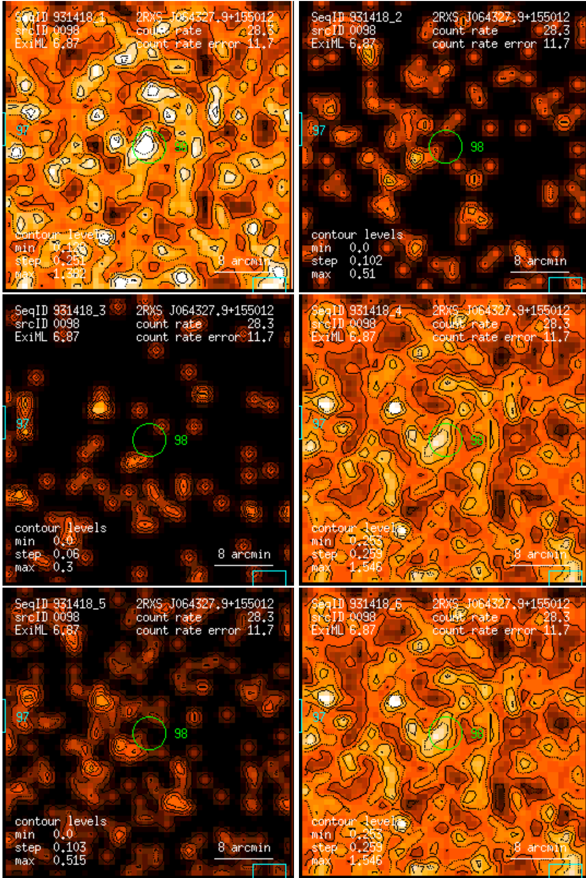
Figure 98: RASS 931418: detection 0098: band rate images, Gaussian filter: (1) PSPC channels 11 – 41, (2) 52 – 90, (3) 91 – 201, (4) 11 – 235, (5) 52 – 201, (6) 11 – 201. Broad band rates in counts/ks. Band rate contour levels in counts/ks/arcmin 2 .
