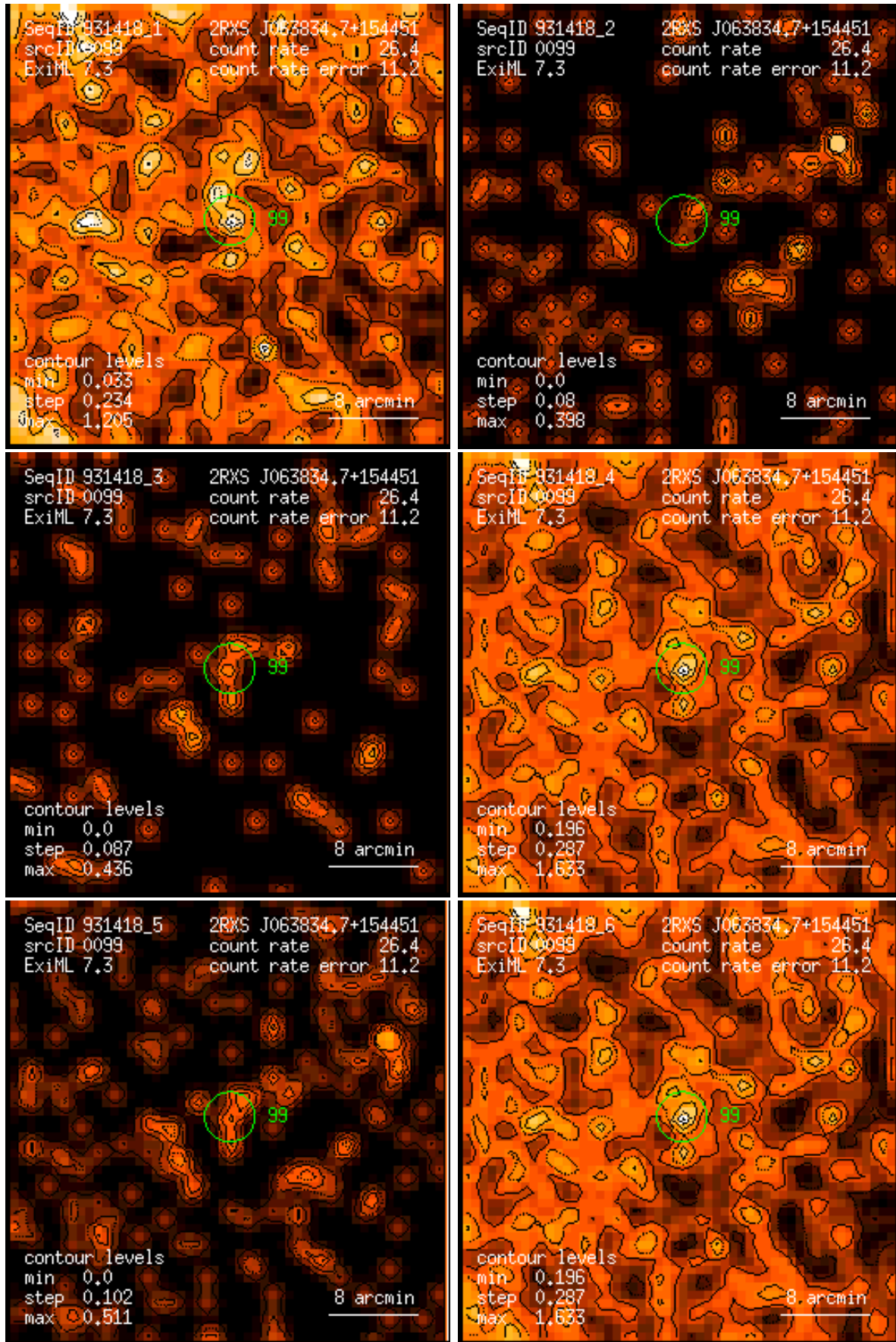
Figure 99: RASS 931418: detection 0099: band rate images, Gaussian filter: (1) PSPC channels 11 – 41, (2) 52 – 90, (3) 91 – 201, (4) 11 – 235, (5) 52 – 201, (6) 11 – 201. Broad band rates in counts/ks. Band rate contour levels in counts/ks/arcmin 2 .
