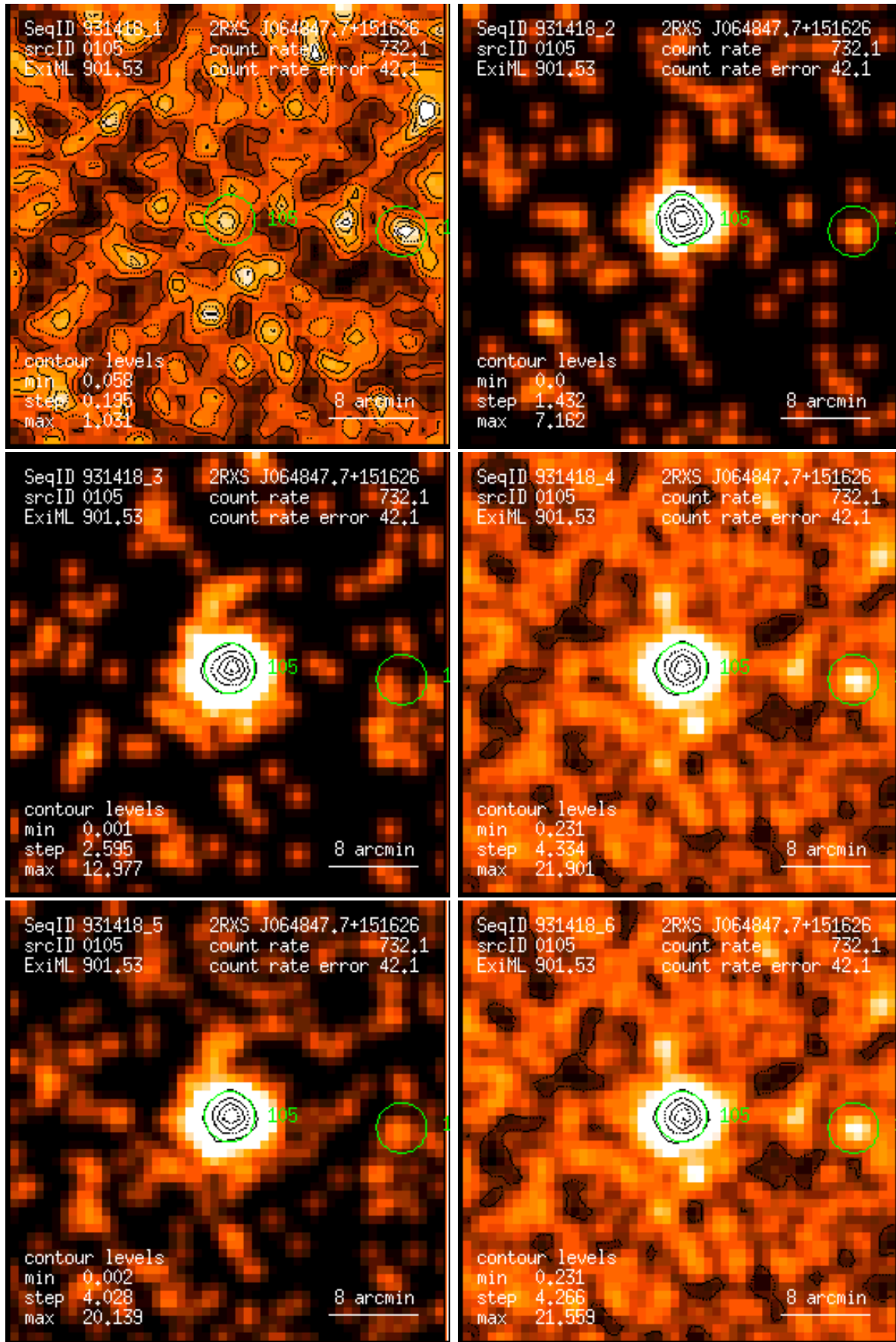
Figure 105: RASS 931418: detection 0105: band rate images, Gaussian filter: (1) PSPC channels 11 – 41, (2) 52 – 90, (3) 91 – 201, (4) 11 – 235, (5) 52 – 201, (6) 11 – 201. Broad band rates in counts/ks. Band rate contour levels in counts/ks/arcmin 2 .
