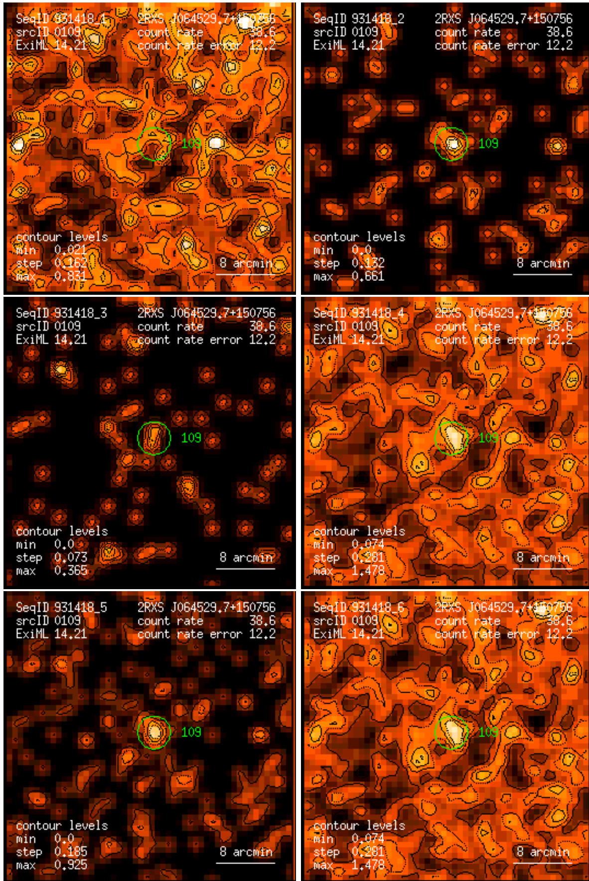
Figure 109: RASS 931418: detection 0109: band rate images, Gaussian filter: (1) PSPC channels 11 – 41, (2) 52 – 90, (3) 91 – 201, (4) 11 – 235, (5) 52 – 201, (6) 11 – 201. Broad band rates in counts/ks. Band rate contour levels in counts/ks/arcmin 2 .
