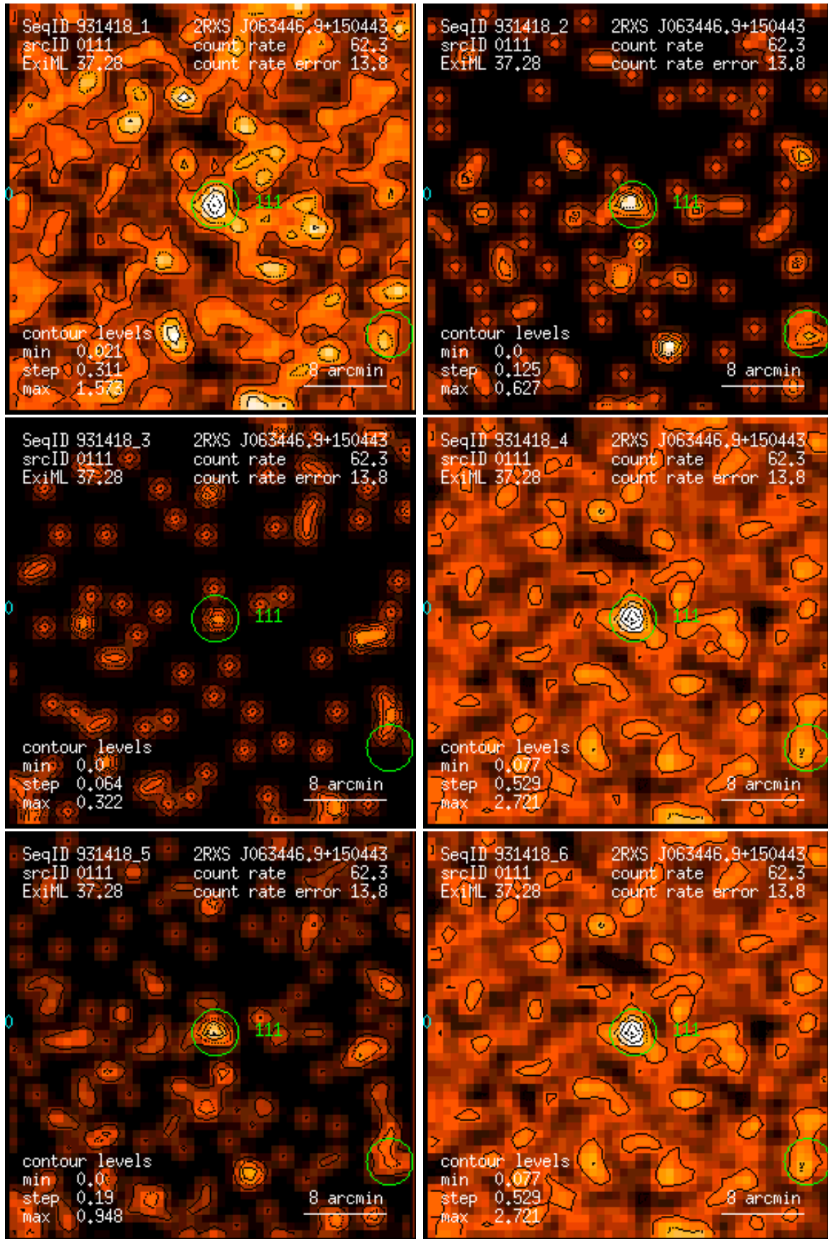
Figure 111: RASS 931418: detection 0111: band rate images, Gaussian filter: (1) PSPC channels 11 – 41, (2) 52 – 90, (3) 91 – 201, (4) 11 – 235, (5) 52 – 201, (6) 11 – 201. Broad band rates in counts/ks. Band rate contour levels in counts/ks/arcmin 2 .
