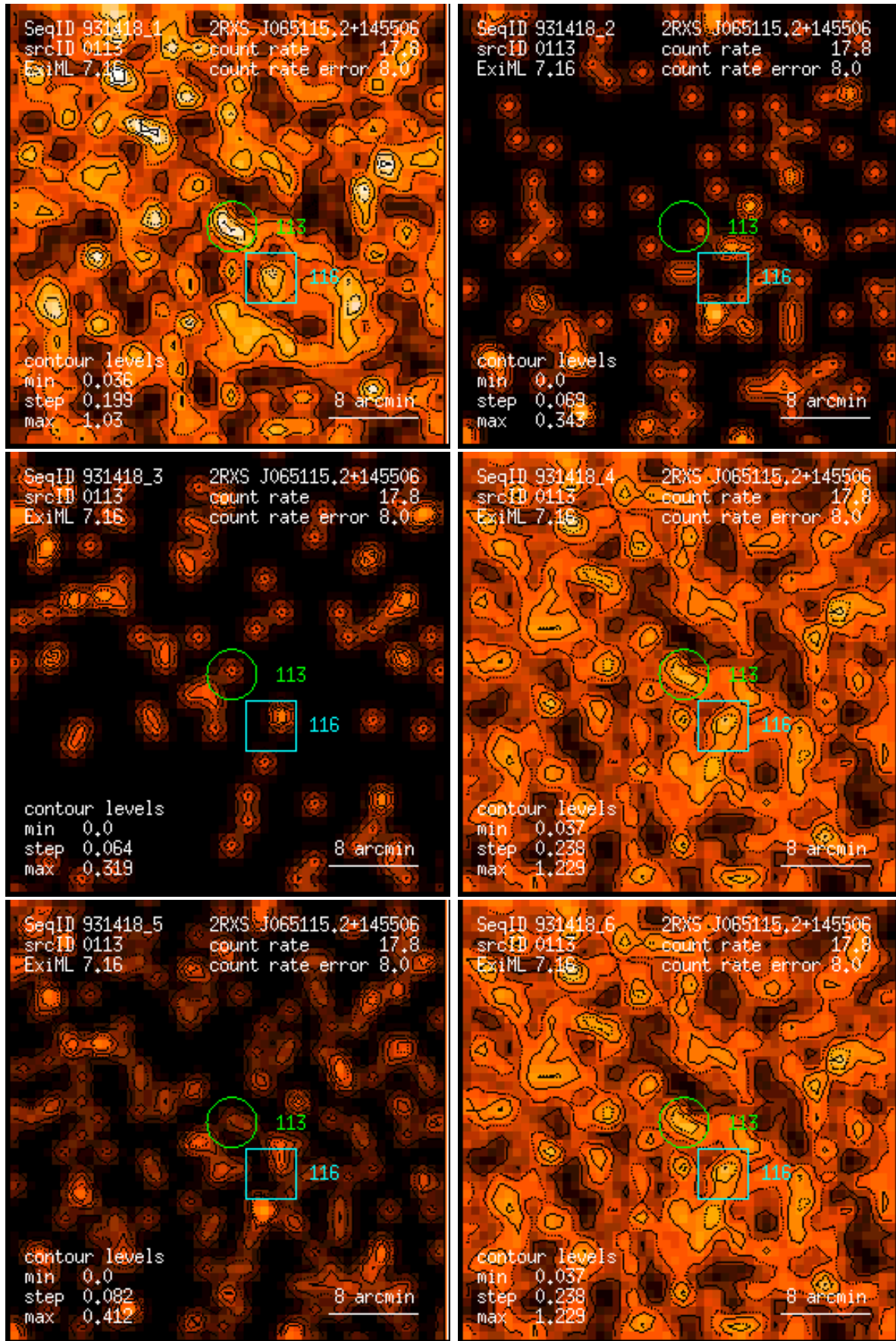
Figure 113: RASS 931418: detection 0113: band rate images, Gaussian filter: (1) PSPC channels 11 – 41, (2) 52 – 90, (3) 91 – 201, (4) 11 – 235, (5) 52 – 201, (6) 11 – 201. Broad band rates in counts/ks. Band rate contour levels in counts/ks/arcmin 2 .
