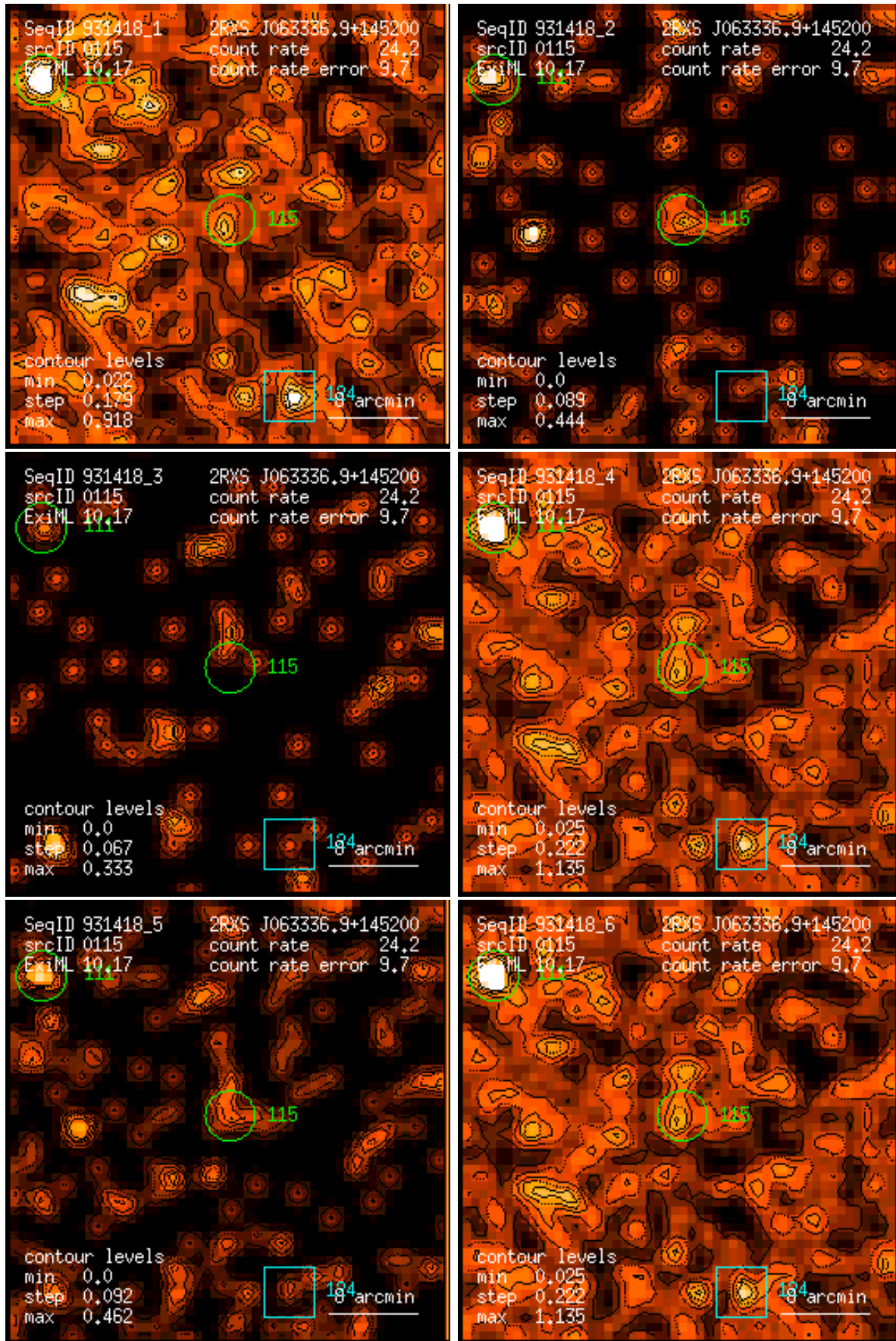
Figure 115: RASS 931418: detection 0115: band rate images, Gaussian filter: (1) PSPPC channels 11 – 41, (2) 52 – 90, (3) 91 – 201, (4) 11 – 235, (5) 52 – 201, (6) 11 – 201. Broad band rates in counts/ks. Band rate contour levels in counts/ks/arcmin 2 .
