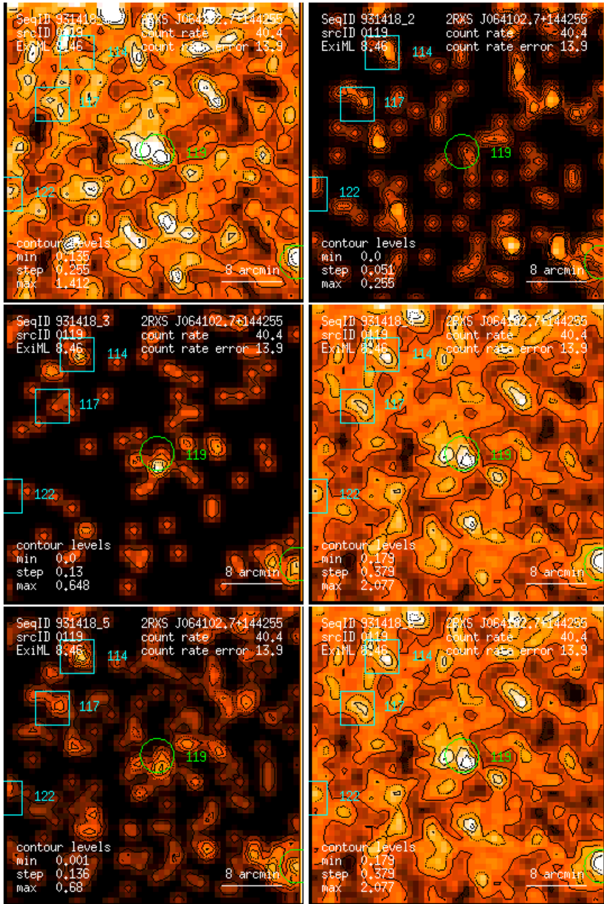
Figure 119: RASS 931418: detection 0119: band rate images, Gaussian filter: (1) PSPC channels 11 – 41, (2) 52 – 90, (3) 91 – 201, (4) 11 – 235, (5) 52 – 201, (6) 11 – 201. Broad band rates in counts/ks. Band rate contour levels in counts/ks/arcmin 2 .
