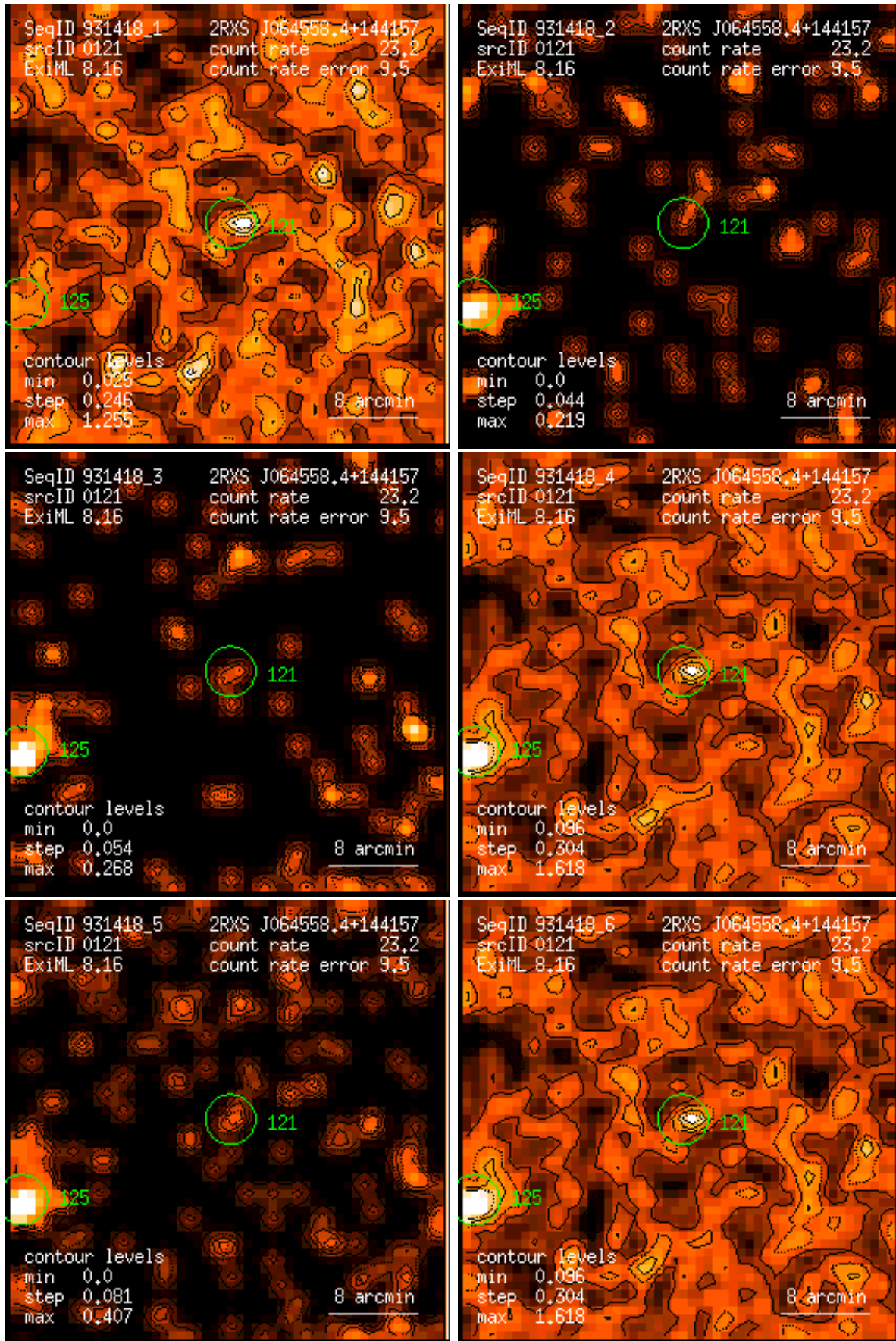
Figure 121: RASS 931418: detection 0121: band rate images, Gaussian filter: (1) PSPC channels 11 – 41, (2) 52 – 90, (3) 91 – 201, (4) 11 – 235, (5) 52 – 201, (6) 11 – 201. Broad band rates in counts/ks. Band rate contour levels in counts/ks/arcmin 2 .
