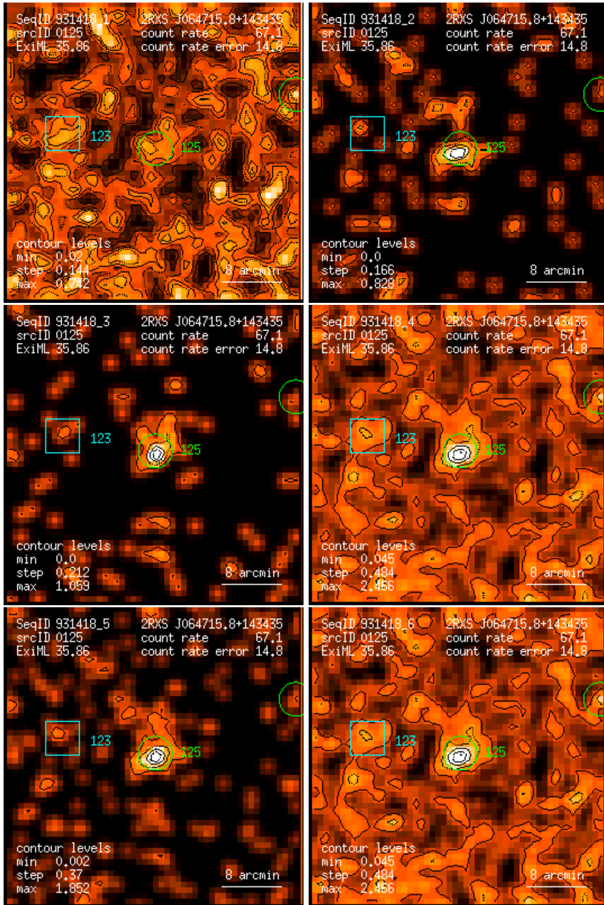
Figure 125: RASS 931418: detection 0125: band rate images, Gaussian filter: (1) PSPC channels 11 – 41, (2) 52 – 90, (3) 91 – 201, (4) 11 – 235, (5) 52 – 201, (6) 11 – 201. Broad band rates in counts/ks. Band rate contour levels in counts/ks/arcmin 2 .
