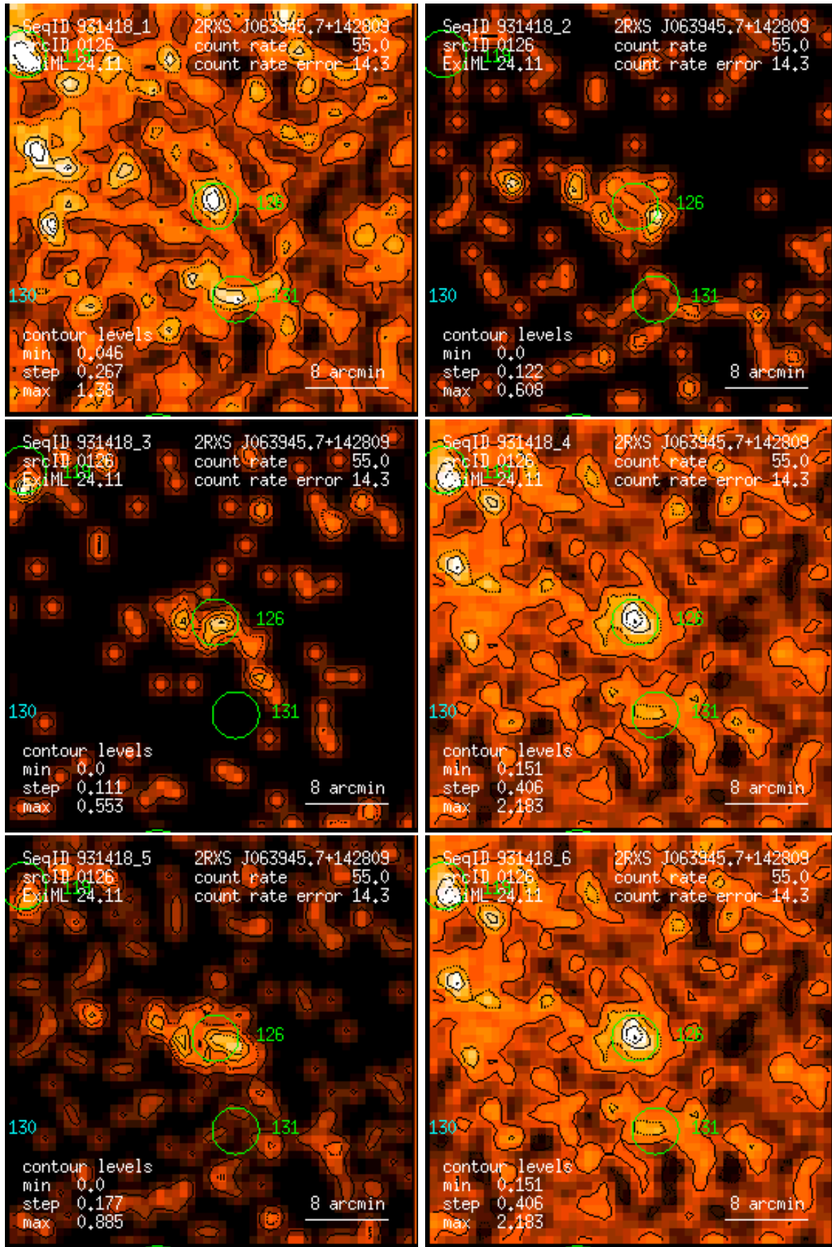
Figure 126: RASS 931418: detection 0126: band rate images, Gaussian filter: (1) PSPC channels 11 – 41, (2) 52 – 90, (3) 91 – 201, (4) 11 – 235, (5) 52 – 201, (6) 11 – 201. Broad band rates in counts/ks. Band rate contour levels in counts/ks/arcmin 2 .
