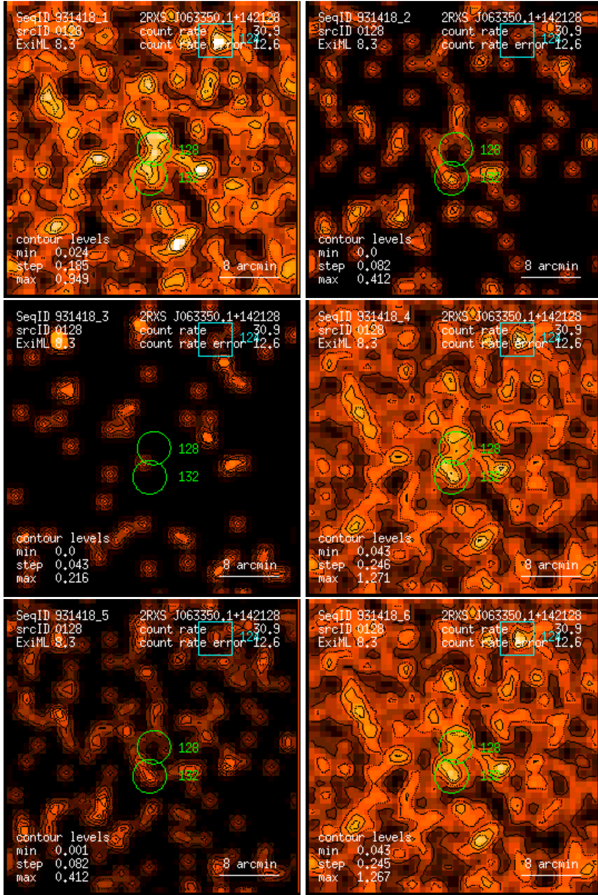
Figure 128: RASS 931418: detection 0128: band rate images, Gaussian filter: (1) PSPC channels 11 – 41, (2) 52 – 90, (3) 91 – 201, (4) 11 – 235, (5) 52 – 201, (6) 11 – 201. Broad band rates in counts/ks. Band rate contour levels in counts/ks/arcmin 2 .
