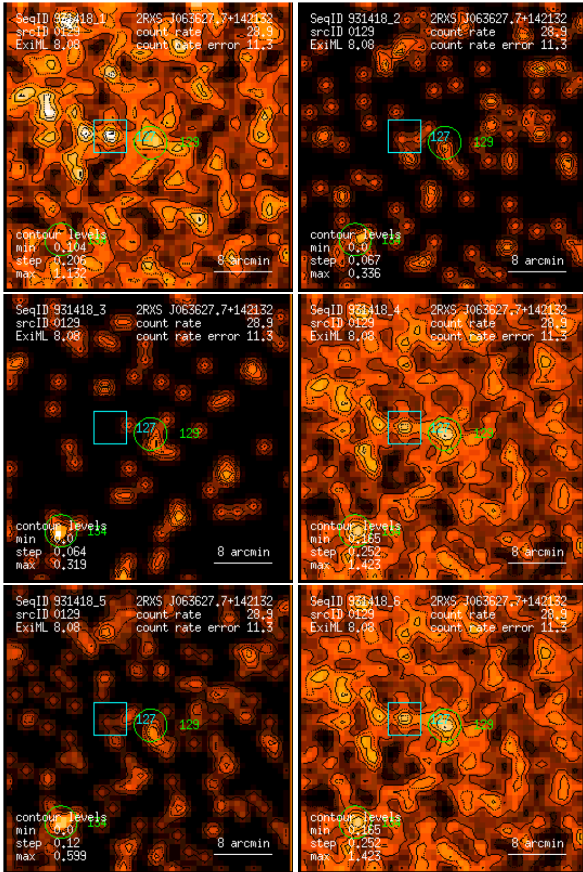
Figure 129: RASS 931418: detection 0129: band rate images, Gaussian filter: (1) PSPC channels 11 – 41, (2) 52 – 90, (3) 91 – 201, (4) 11 – 235, (5) 52 – 201, (6) 11 – 201. Broad band rates in counts/ks. Band rate contour levels in counts/ks/arcmin 2 .
