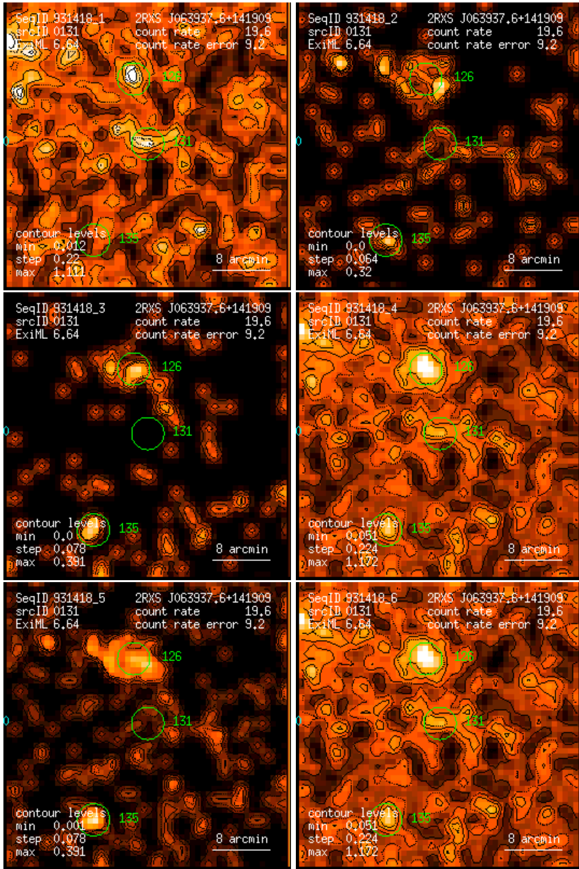
Figure 131: RASS 931418: detection 0131: band rate images, Gaussian filter: (1) PSPC channels 11 – 41, (2) 52 – 90, (3) 91 – 201, (4) 11 – 235, (5) 52 – 201, (6) 11 – 201. Broad band rates in counts/ks. Band rate contour levels in counts/ks/arcmin 2 .
