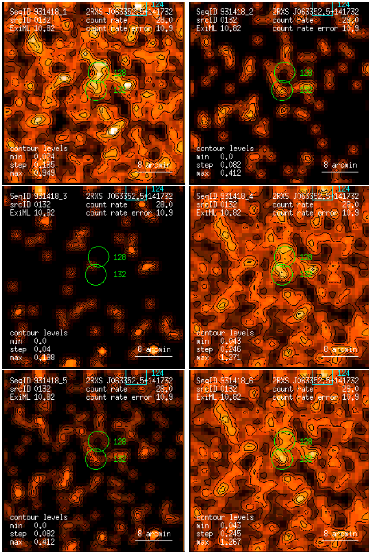
Figure 132: RASS 931418: detection 0132: band rate images, Gaussian filter: (1) PSPC channels 11 – 41, (2) 52 – 90, (3) 91 – 201, (4) 11 – 235, (5) 52 – 201, (6) 11 – 201. Broad band rates in counts/ks. Band rate contour levels in counts/ks/arcmin 2 .
