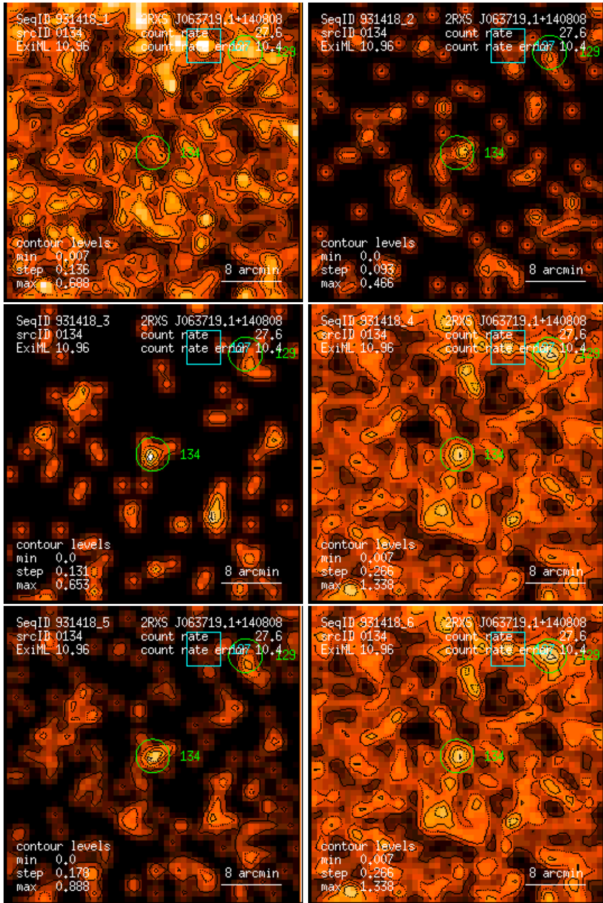
Figure 134: RASS 931418: detection 0134: band rate images, Gaussian filter: (1) PSPC channels 11 – 41, (2) 52 – 90, (3) 91 – 201, (4) 11 – 235, (5) 52 – 201, (6) 11 – 201. Broad band rates in counts/ks. Band rate contour levels in counts/ks/arcmin 2 .
