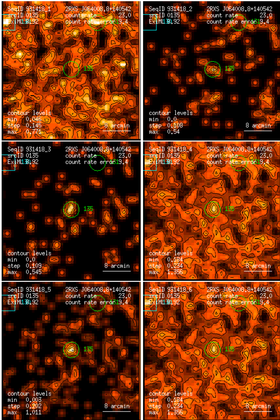
Figure 135: RASS 931418: detection 0135: band rate images, Gaussian filter: (1) PSPC channels 11 – 41, (2) 52 – 90, (3) 91 – 201, (4) 11 – 235, (5) 52 – 201, (6) 11 – 201. Broad band rates in counts/ks. Band rate contour levels in counts/ks/arcmin 2 .
