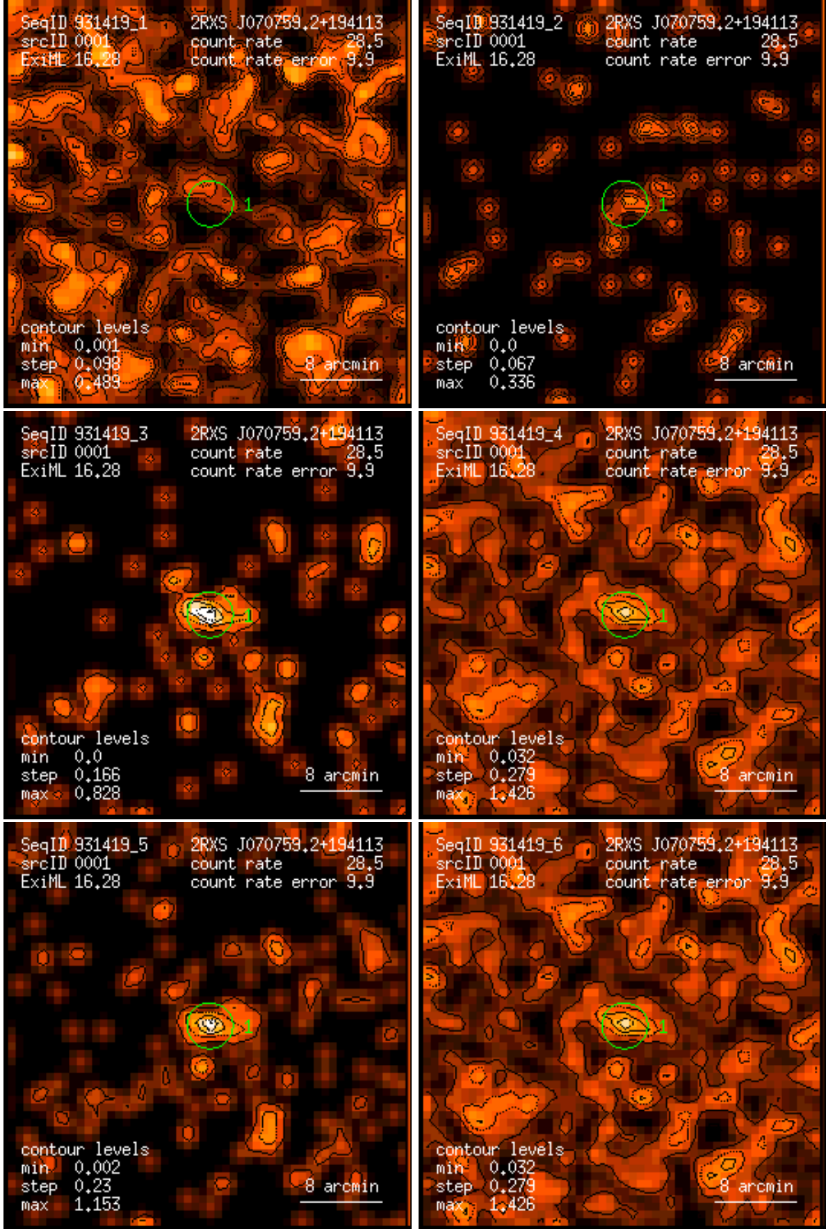
Figure 1: RASS 931419: detection 0001: band rate images, Gaussian filter: (1) PSPC channels 11 – 41, (2) 52 – 90, (3) 91 – 201, (4) 11 – 235, (5) 52 – 201, (6) 11 – 201. Broad band rates in counts/ks. Band rate contour levels in counts/ks/arcmin 2 .
