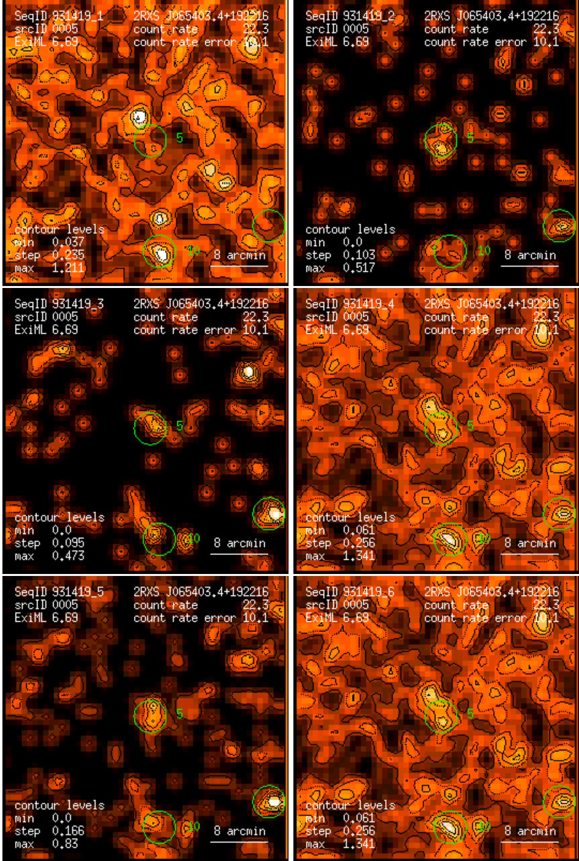
Figure 5: RASS 931419: detection 0005: band rate images, Gaussian filter: (1) PSPC channels 11 – 41, (2) 52 – 90, (3) 91 – 201, (4) 11 – 235, (5) 52 – 201, (6) 11 – 201. Broad band rates in counts/ks. Band rate contour levels in counts/ks/arcmin 2 .
