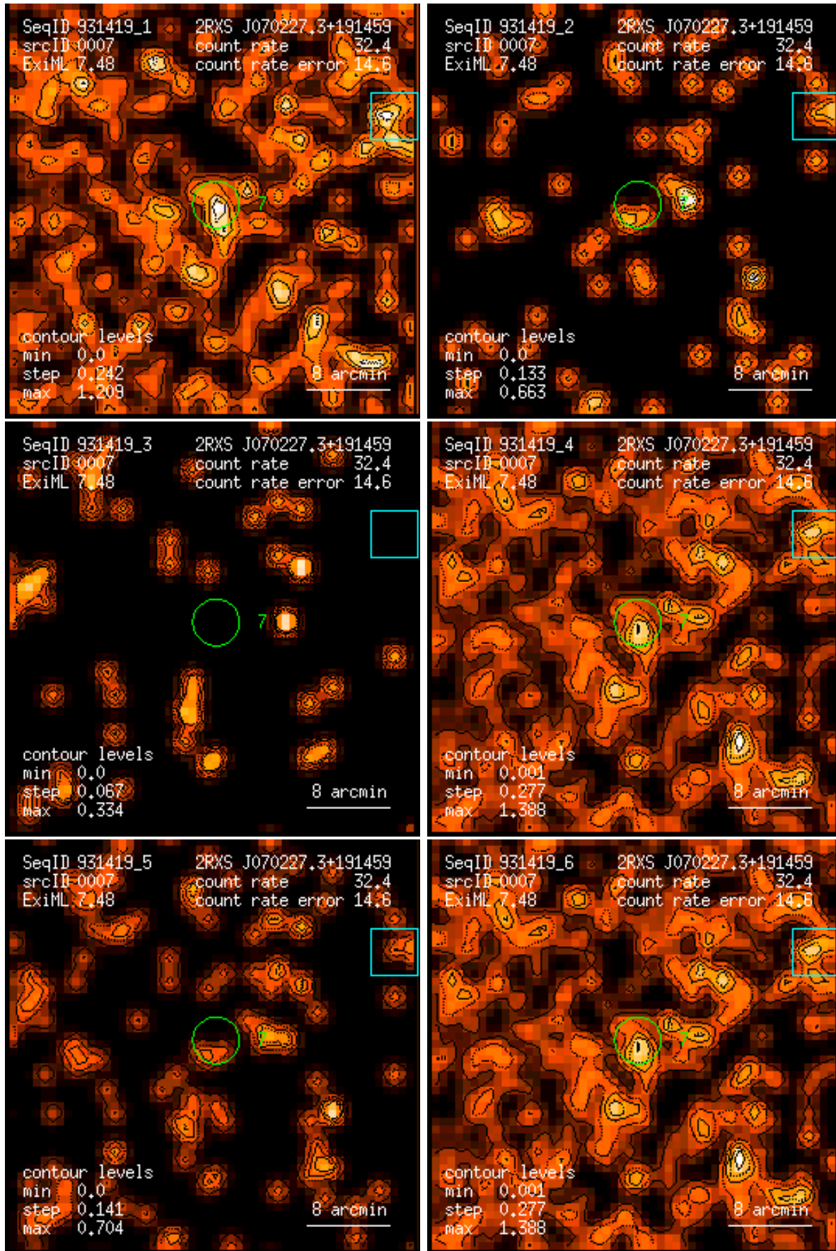
Figure 7: RASS 931419: detection 0007: band rate images, Gaussian filter: (1) PSPC channels 11 – 41, (2) 52 – 90, (3) 91 – 201, (4) 11 – 235, (5) 52 – 201, (6) 11 – 201. Broad band rates in counts/ks. Band rate contour levels in counts/ks/arcmin 2 .
