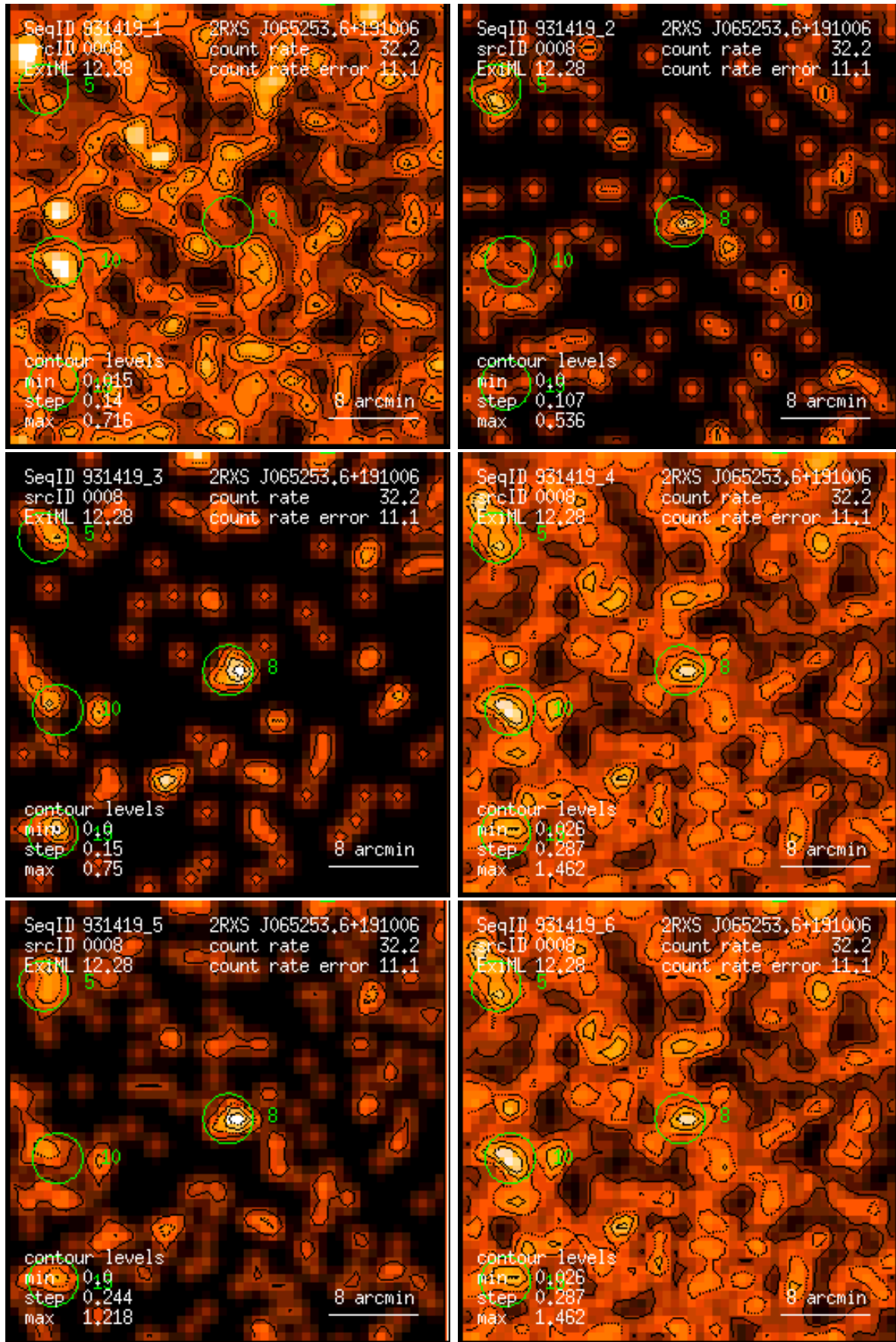
Figure 8: RASS 931419: detection 0008: band rate images, Gaussian filter: (1) PSPC channels 11 – 41, (2) 52 – 90, (3) 91 – 201, (4) 11 – 235, (5) 52 – 201, (6) 11 – 201. Broad band rates in counts/ks. Band rate contour levels in counts/ks/arcmin 2 .
