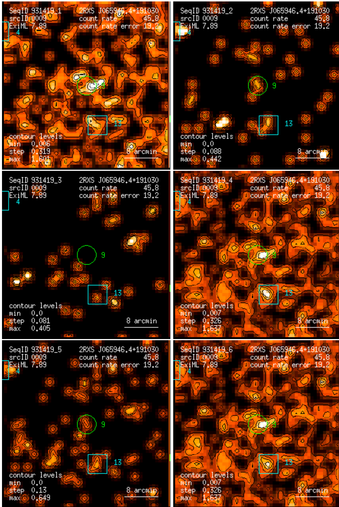
Figure 9: RASS 931419: detection 0009: band rate images, Gaussian filter: (1) PSPC channels 11 – 41, (2) 52 – 90, (3) 91 – 201, (4) 11 – 235, (5) 52 – 201, (6) 11 – 201. Broad band rates in counts/ks. Band rate contour levels in counts/ks/arcmin 2 .
