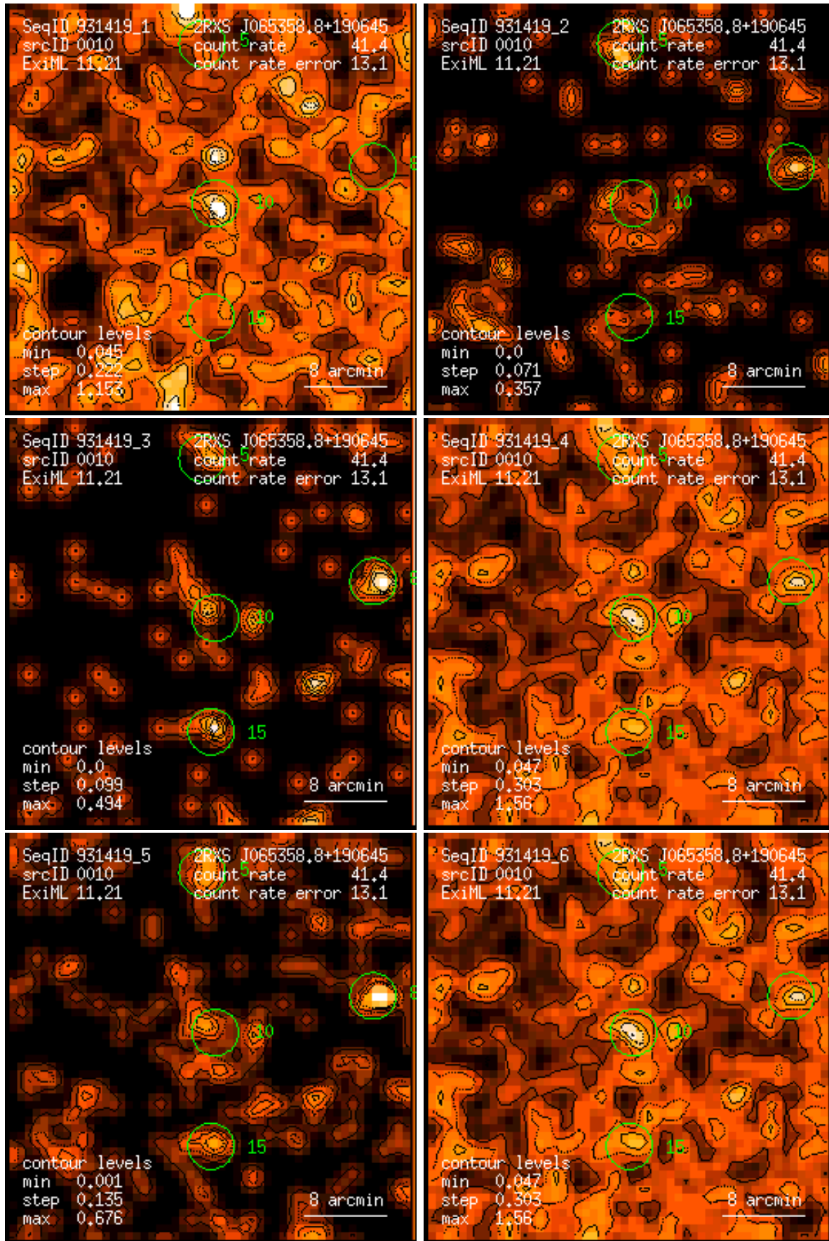
Figure 10: RASS 931419: detection 0010: band rate images, Gaussian filter: (1) PSPC channels 11 – 41, (2) 52 – 90, (3) 91 – 201, (4) 11 – 235, (5) 52 – 201, (6) 11 – 201. Broad band rates in counts/ks. Band rate contour levels in counts/ks/arcmin 2 .
