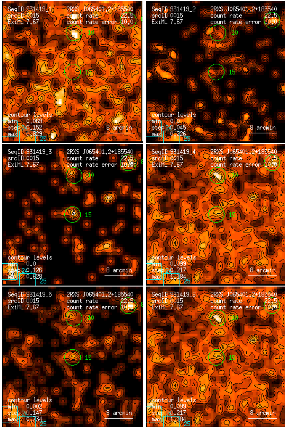
Figure 15: RASS 931419: detection 0015: band rate images, Gaussian filter: (1) PSPC channels 11 – 41, (2) 52 – 90, (3) 91 – 201, (4) 11 – 235, (5) 52 – 201, (6) 11 – 201. Broad band rates in counts/ks. Band rate contour levels in counts/ks/arcmin 2 .
