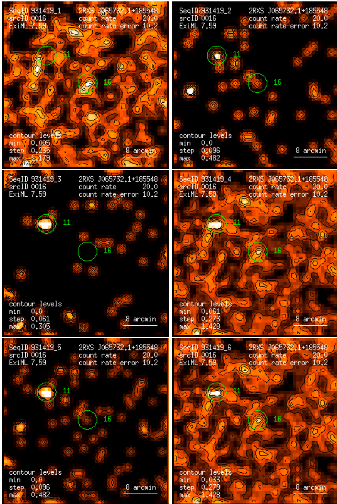
Figure 16: RASS 931419: detection 0016: band rate images, Gaussian filter: (1) PSPC channels 11 – 41, (2) 52 – 90, (3) 91 – 201, (4) 11 – 235, (5) 52 – 201, (6) 11 – 201. Broad band rates in counts/ks. Band rate contour levels in counts/ks/arcmin 2 .
