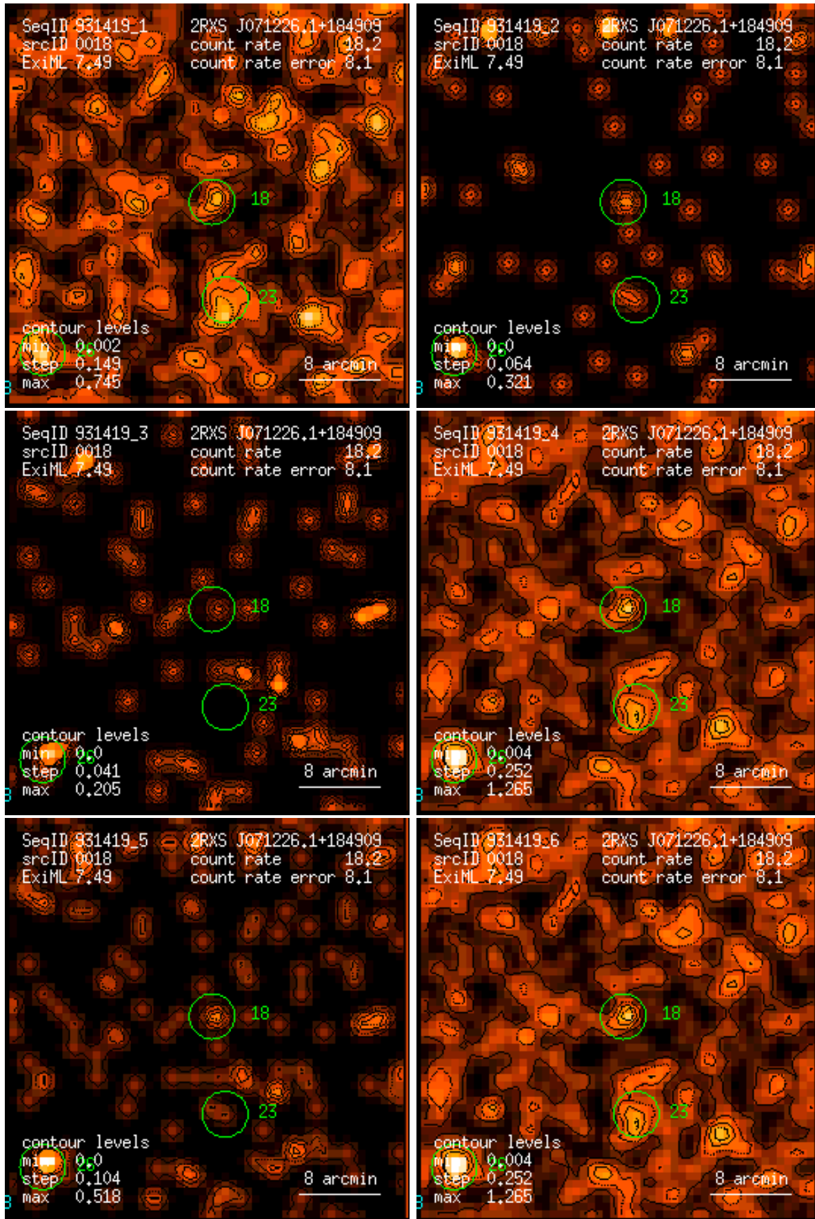
Figure 18: RASS 931419: detection 0018: band rate images, Gaussian filter: (1) PSPC channels 11 – 41, (2) 52 – 90, (3) 91 – 201, (4) 11 – 235, (5) 52 – 201, (6) 11 – 201. Broad band rates in counts/ks. Band rate contour levels in counts/ks/arcmin 2 .
