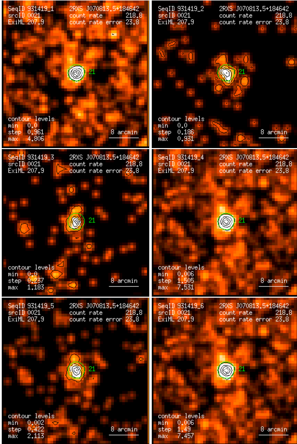
Figure 21: RASS 931419: detection 0021: band rate images, Gaussian filter: (1) PSPC channels 11 – 41, (2) 52 – 90, (3) 91 – 201, (4) 11 – 235, (5) 52 – 201, (6) 11 – 201. Broad band rates in counts/ks. Band rate contour levels in counts/ks/arcmin 2 .
