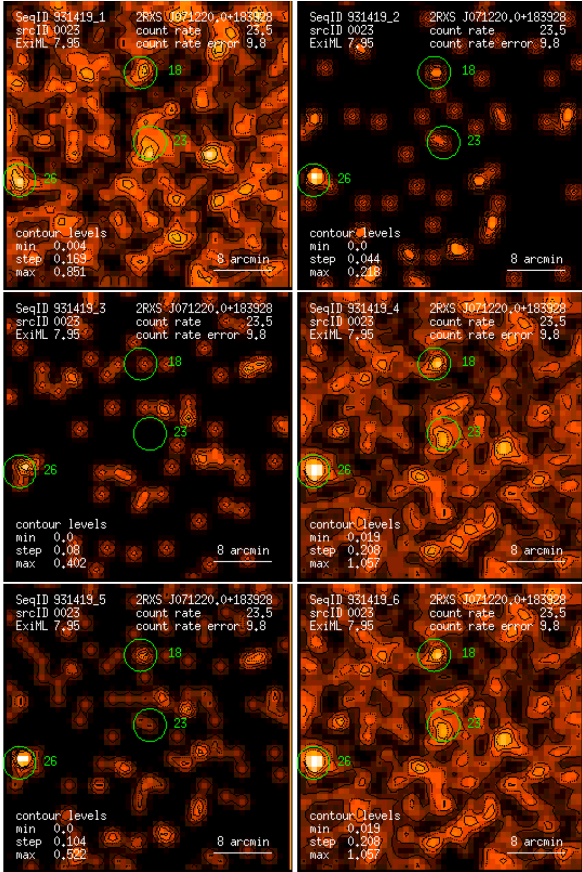
Figure 23: RASS 931419: detection 0023: band rate images, Gaussian filter: (1) PSPC channels 11 – 41, (2) 52 – 90, (3) 91 – 201, (4) 11 – 235, (5) 52 – 201, (6) 11 – 201. Broad band rates in counts/ks. Band rate contour levels in counts/ks/arcmin 2 .
