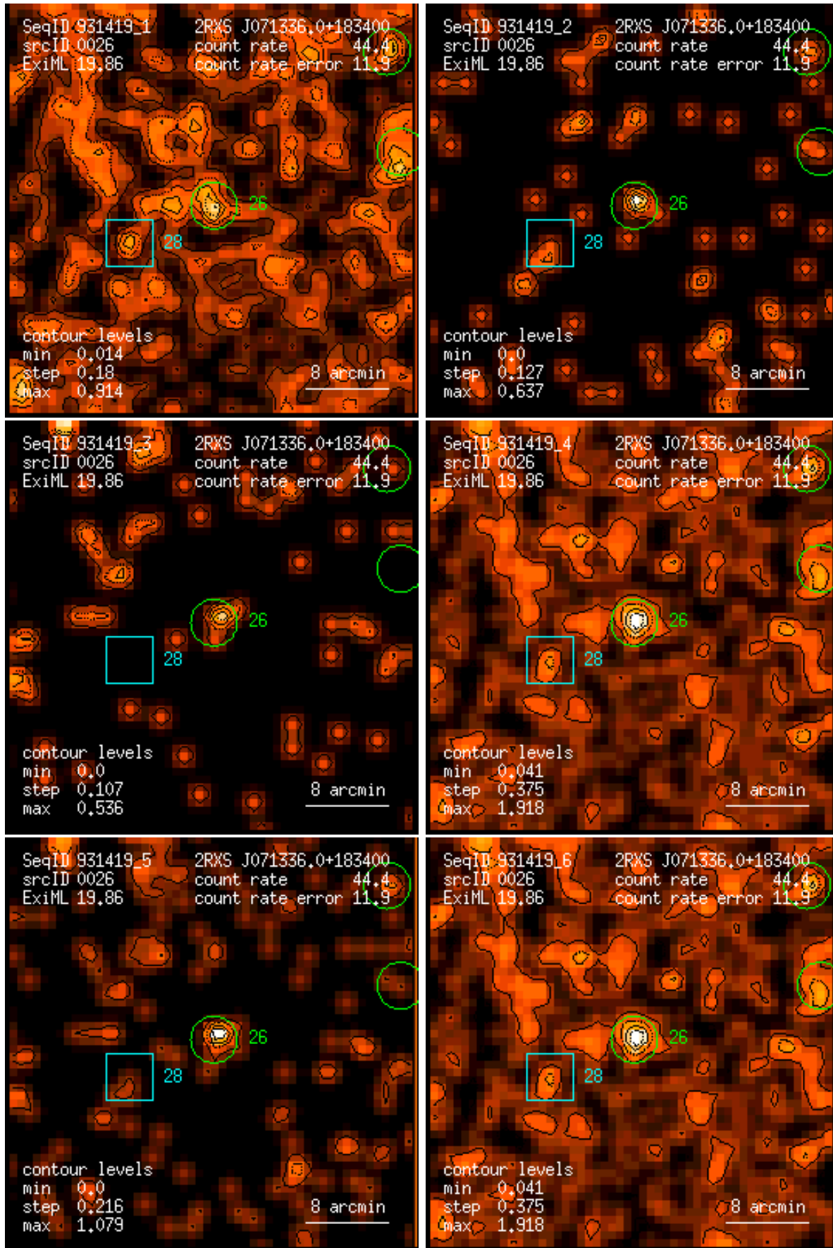
Figure 26: RASS 931419: detection 0026: band rate images, Gaussian filter: (1) PSPC channels 11 – 41, (2) 52 – 90, (3) 91 – 201, (4) 11 – 235, (5) 52 – 201, (6) 11 – 201. Broad band rates in counts/ks. Band rate contour levels in counts/ks/arcmin 2 .
