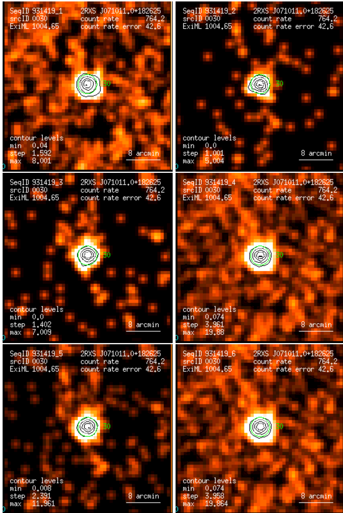
Figure 30: RASS 931419: detection 0030: band rate images, Gaussian filter: (1) PSPC channels 11 – 41, (2) 52 – 90, (3) 91 – 201, (4) 11 – 235, (5) 52 – 201, (6) 11 – 201. Broad band rates in counts/ks. Band rate contour levels in counts/ks/arcmin 2 .
