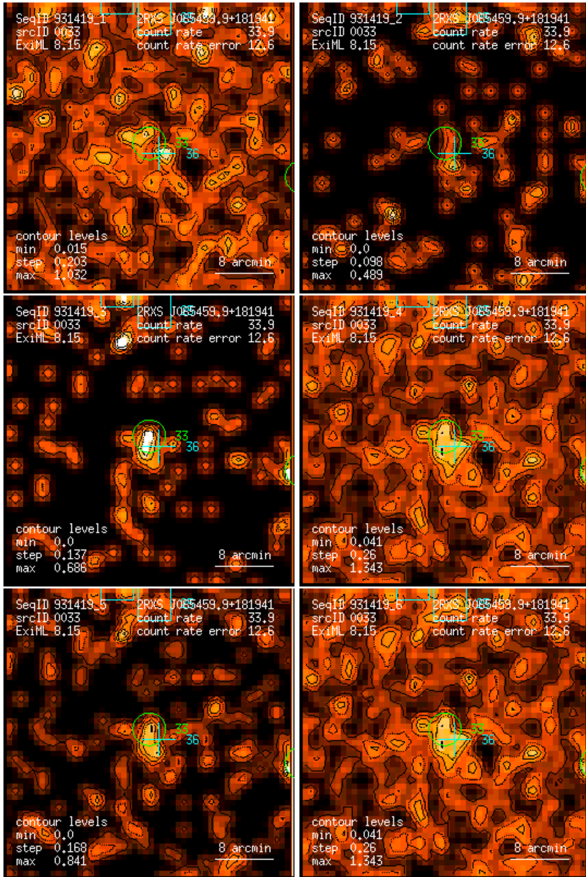
Figure 33: RASS 931419: detection 0033: band rate images, Gaussian filter: (1) PSPC channels 11 – 41, (2) 52 – 90, (3) 91 – 201, (4) 11 – 235, (5) 52 – 201, (6) 11 – 201. Broad band rates in counts/ks. Band rate contour levels in counts/ks/arcmin 2 .
